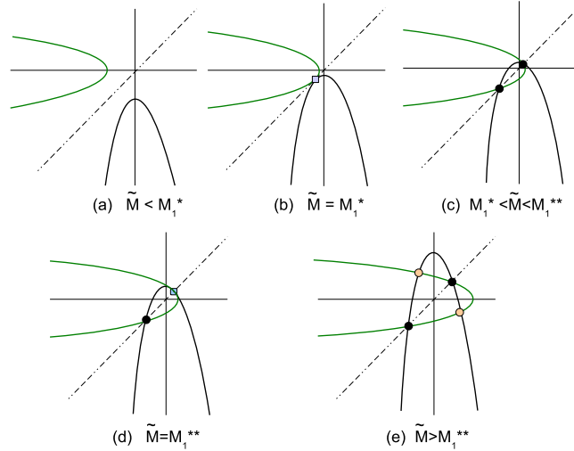
Figure 6. A geometric interpretation of the fixed points of map H in (3.13) as intersection points of a symmetric couple of parabolas (case \tilde{c} < 1 )
