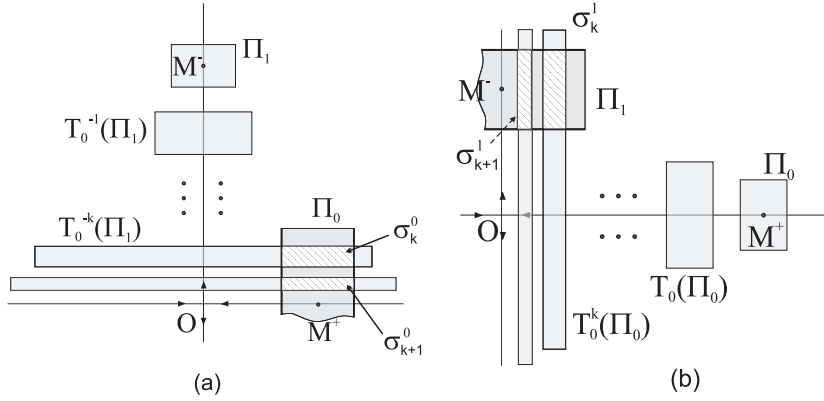
Figure 5. A geometry of creation of both domains of definition \sigma_i^0 \subset \Pi^+ (a) and domains of the range \sigma_i^1 \subset \Pi^- (b) for the maps T_0^i : \Pi^+ \rightarrow \Pi^- .
