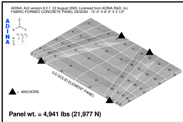
Figure 8: Panel model
