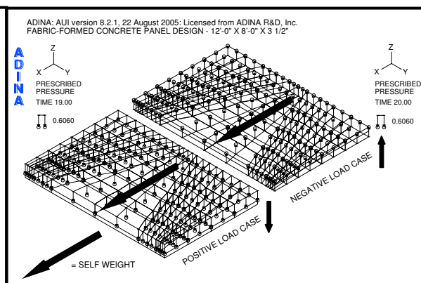
Figure 7: Panel load cases. (1 psi = 6.9 kPa)
