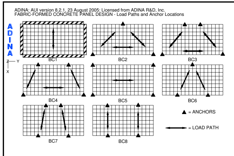
Figure 3: Panel load paths and anchor locations
