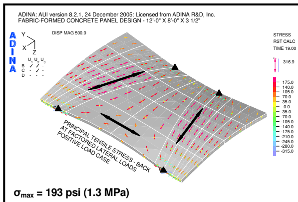
Figure 14: Panel principal stresses, back
