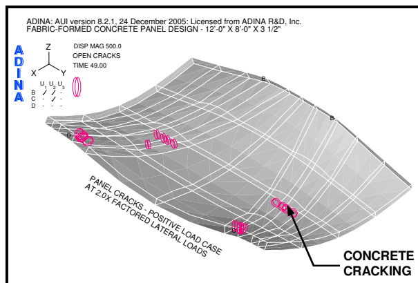
Figure 10: First panel cracks, back.
