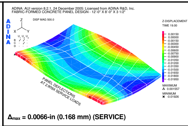
Figure 9: Panel deflections
