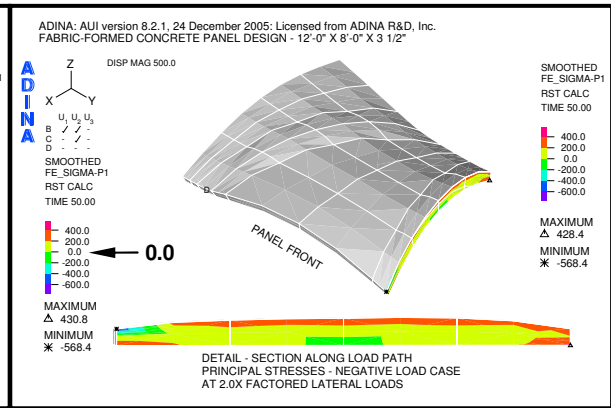
Figure 13: Principal stresses at section cut
