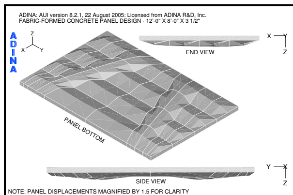
Figure 6: Panel shape after “form-finding”
