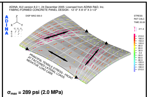
Figure 15: Panel principal stresses, front
