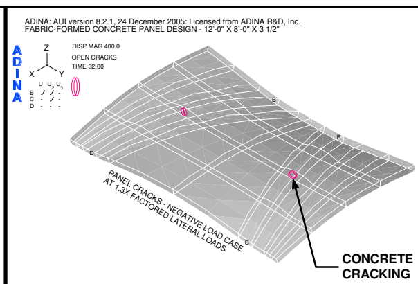
Figure 11: First panel cracks, front.
