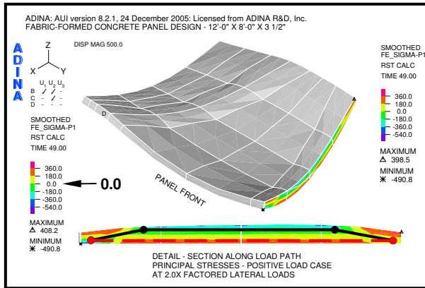
Figure 12: Principal stresses at section cut
