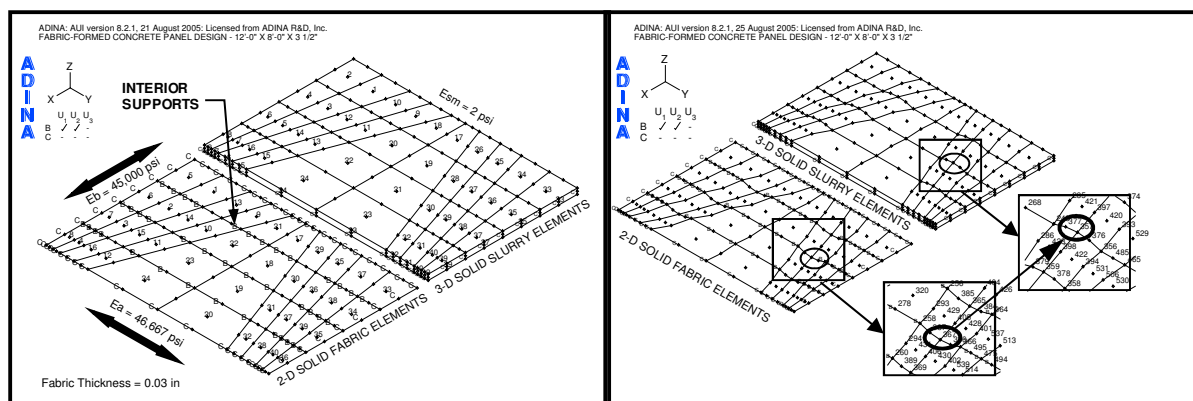
Figure 4: Combined fabric and slurry model (1-in = 25.4 mm, 1 psi = 6.9 kPa)
