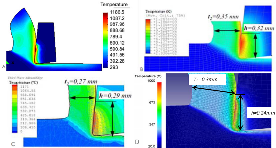
Fig. 2. Comparisons of temperature fields given by A. PFEM, B. Abaqus, C. AdvantEdge and D. Deform.
