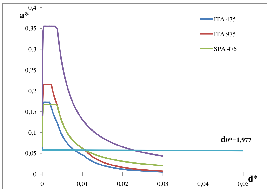
Figure A.19 – Capacity curve and demand spectrums of mechanism 7.
