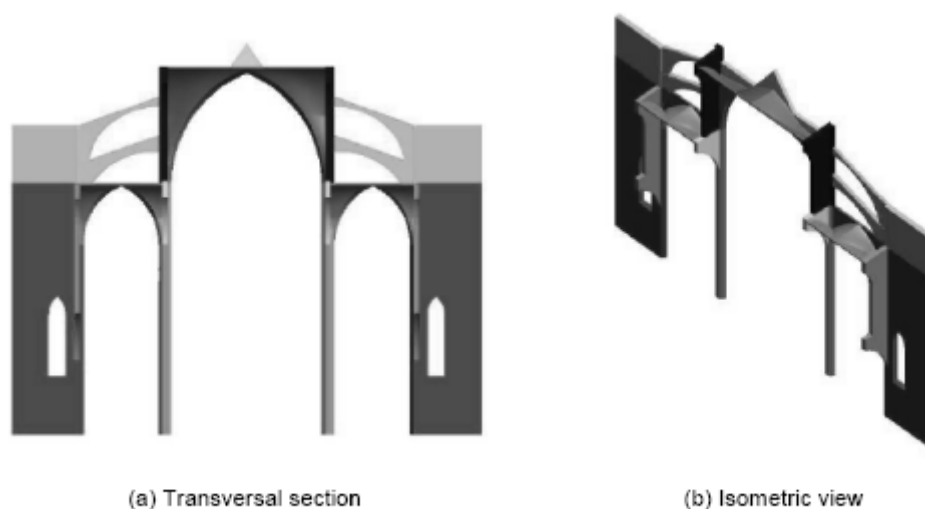
Figure 4.16 – Geometry of the bay of Mallorca cathedral (Das 2008)
