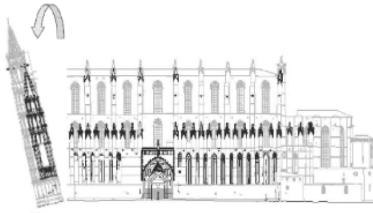
Example of a collapse mechanism of Mallorca Cathedral (Cuzzilla (2008)).
