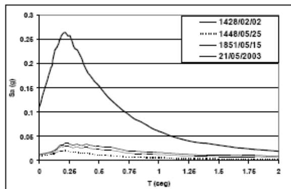
Deterministic scenario spectrums according to Martinez (2007).
