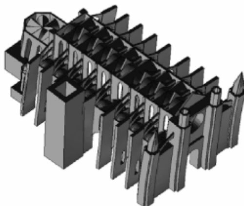
First mode of vibration obtained by the modelling carried out by Martinez (2007).
