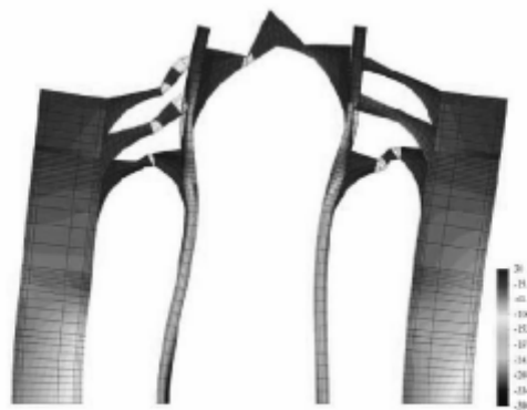
Distribution of normal stresses, cracking and deformation of the generalized matrix formulation model corresponding to a wind pressure of 1.45kN/m 2 (Salas (2002)).
