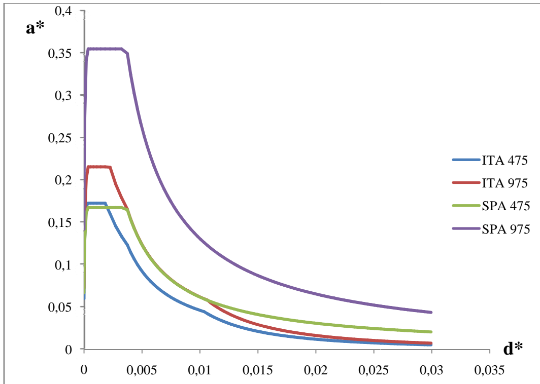
Figure 5.20 – Comparison between the different seismic demands for Mallorca Cathedral.
