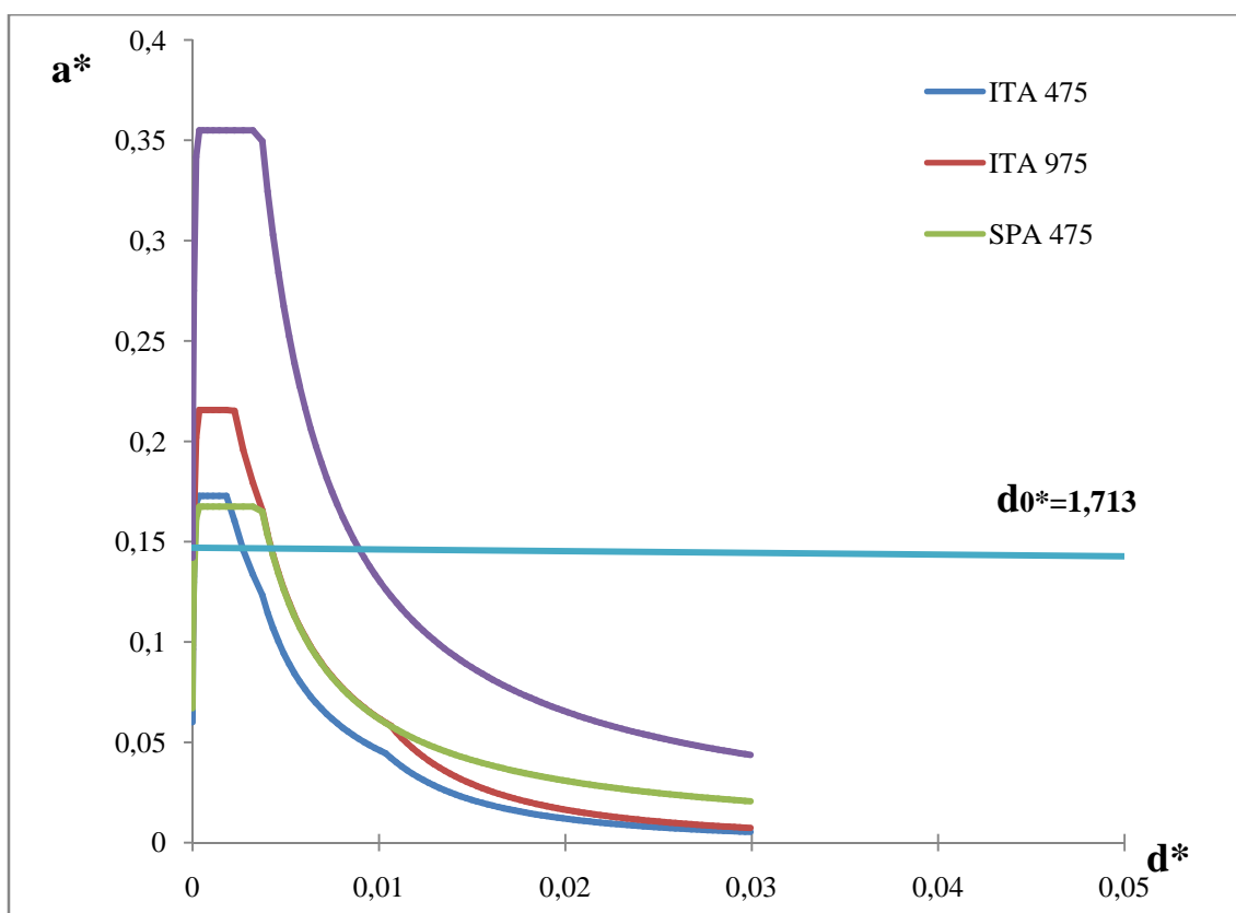
Figure A.13 – Capacity curve and demand spectrums of mechanism 4.
