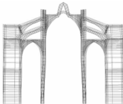
Deformed shape of the generalized matrix formulation model without the extra weights corresponding to a gravity load factor of 0.9 (Salas (2002)).
