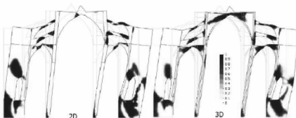
Collapse mechanism and tension damage obtained with seismic analysis (Clemente (2006)).
