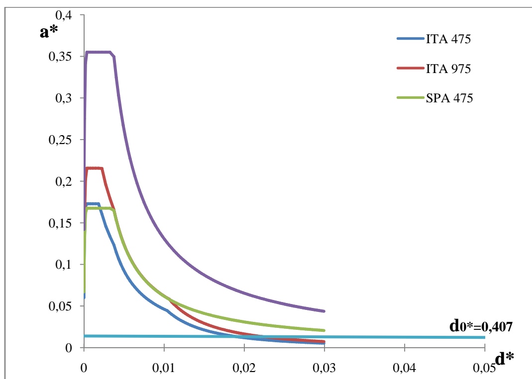
Figure A.31 – Capacity curve and demand spectrums of mechanism 14.
