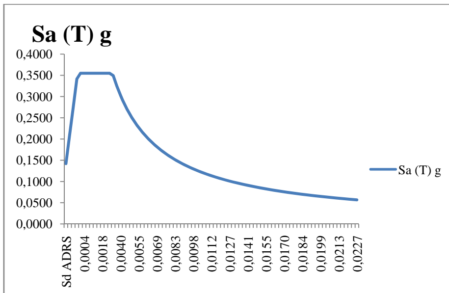
Figure 5.17 - Graph in the ADRS format
