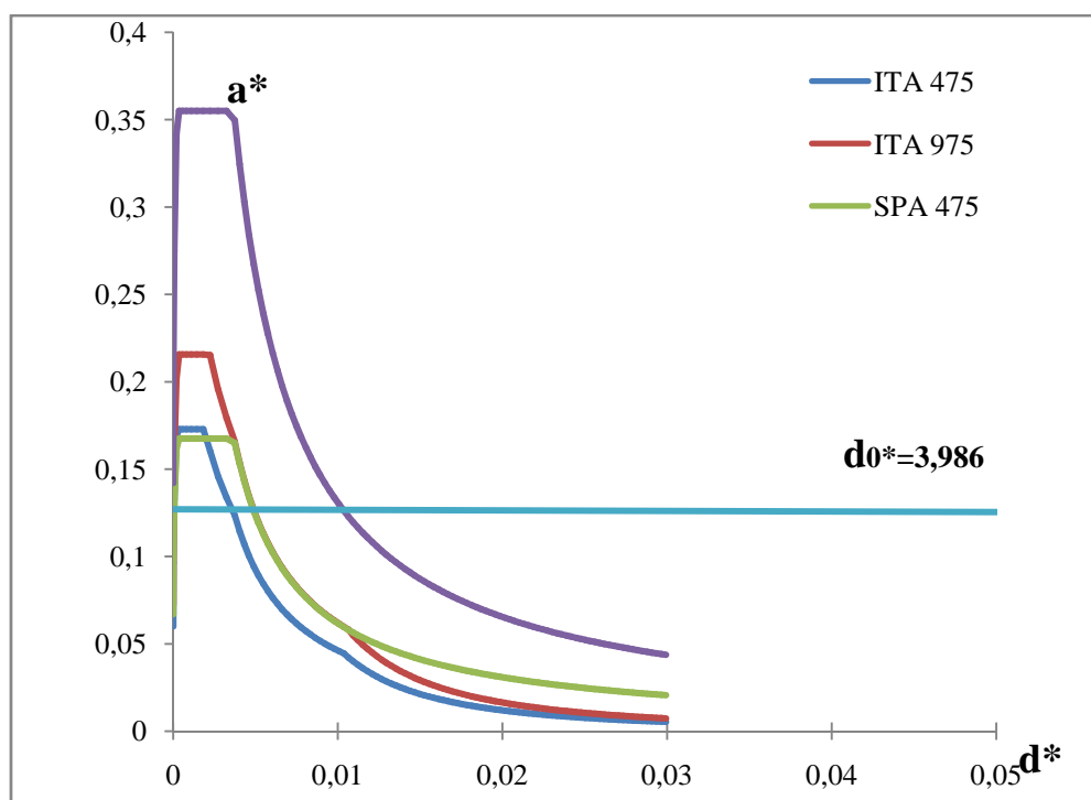
Figure A.7 – Capacity curve and demand spectrums of mechanism 1.
