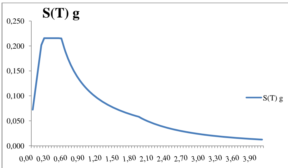
Figure 5.18 – Response spectrum
