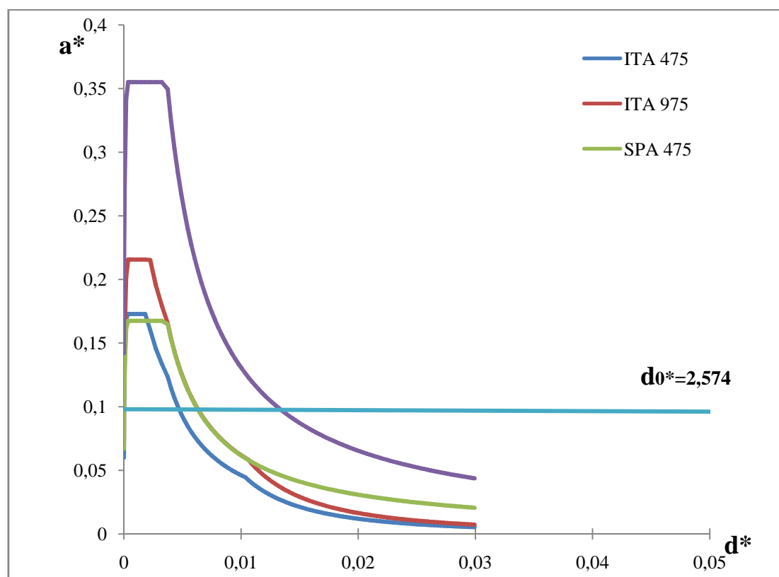
Figure A.23 – Capacity curve and demand spectrums of mechanism 9.
