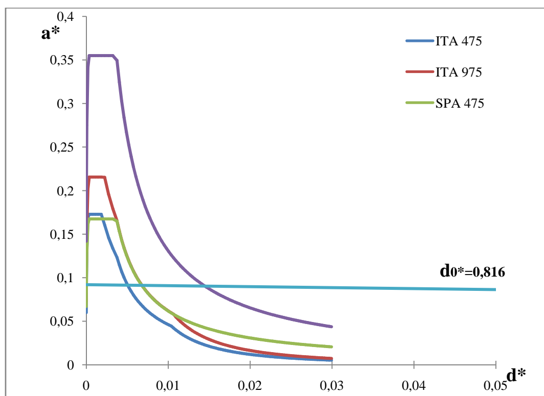
Figure A.27 – Capacity curve and demand spectrums of mechanism 11.
