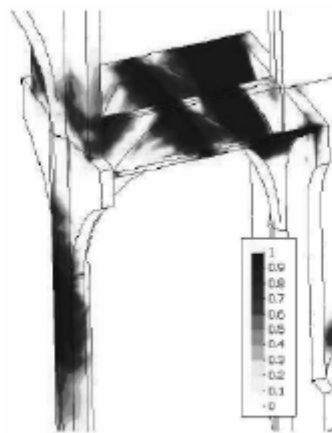
Distribution of tension in collapse due to creep effect (Clemente (2006)).
