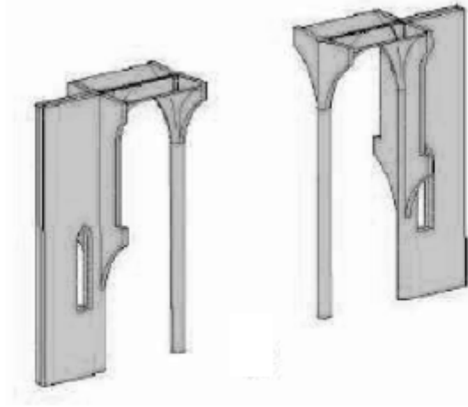
First phase of the construction process simulated by (Clemente (2006)).
