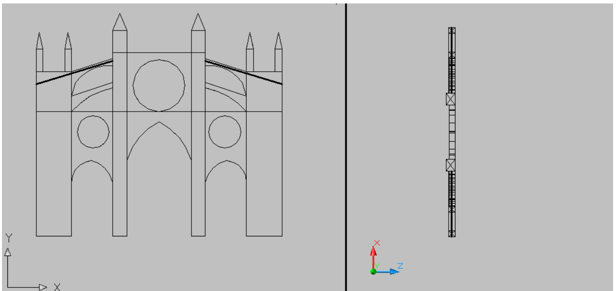
Figure 6.2 – Strengthening solution for mechanism 11 and 14.
