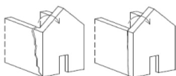
(a) Façade overturning
