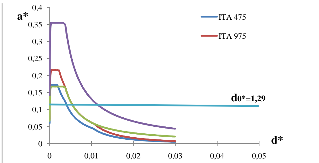
Figure A.5 – Capacity curve and demand spectrums of mechanism 13.
