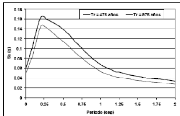
Response spectra of uniform hazard on firm soil for return periods equal to 475 and 975 years according to Martinez (2007).
