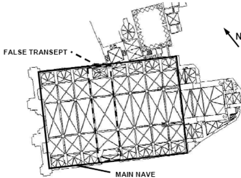
Figure 3.2 – Plan of Mallorca Cathedral.
