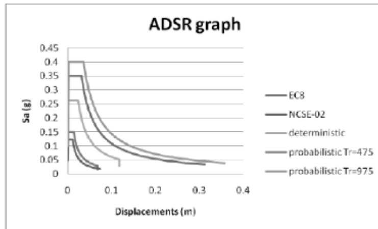
Figure 4.19 - ADRS
