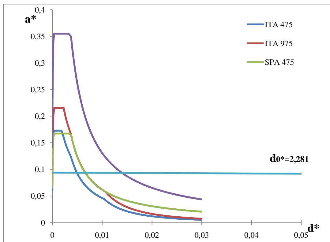
Figure A.29 – Capacity curve and demand spectrum of mechanism 12.
