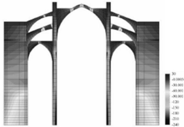
Stresses of the generalized matrix formulation model without the extra weights corresponding to a gravity load factor of 0.9 (Salas (2002)).
