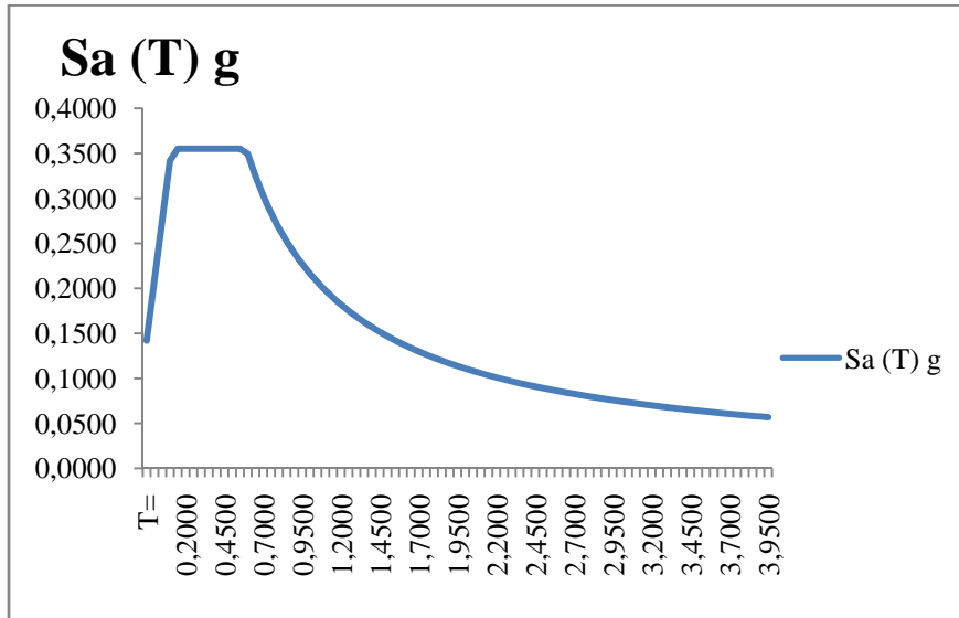
Figure 5.16 - Response spectrum
