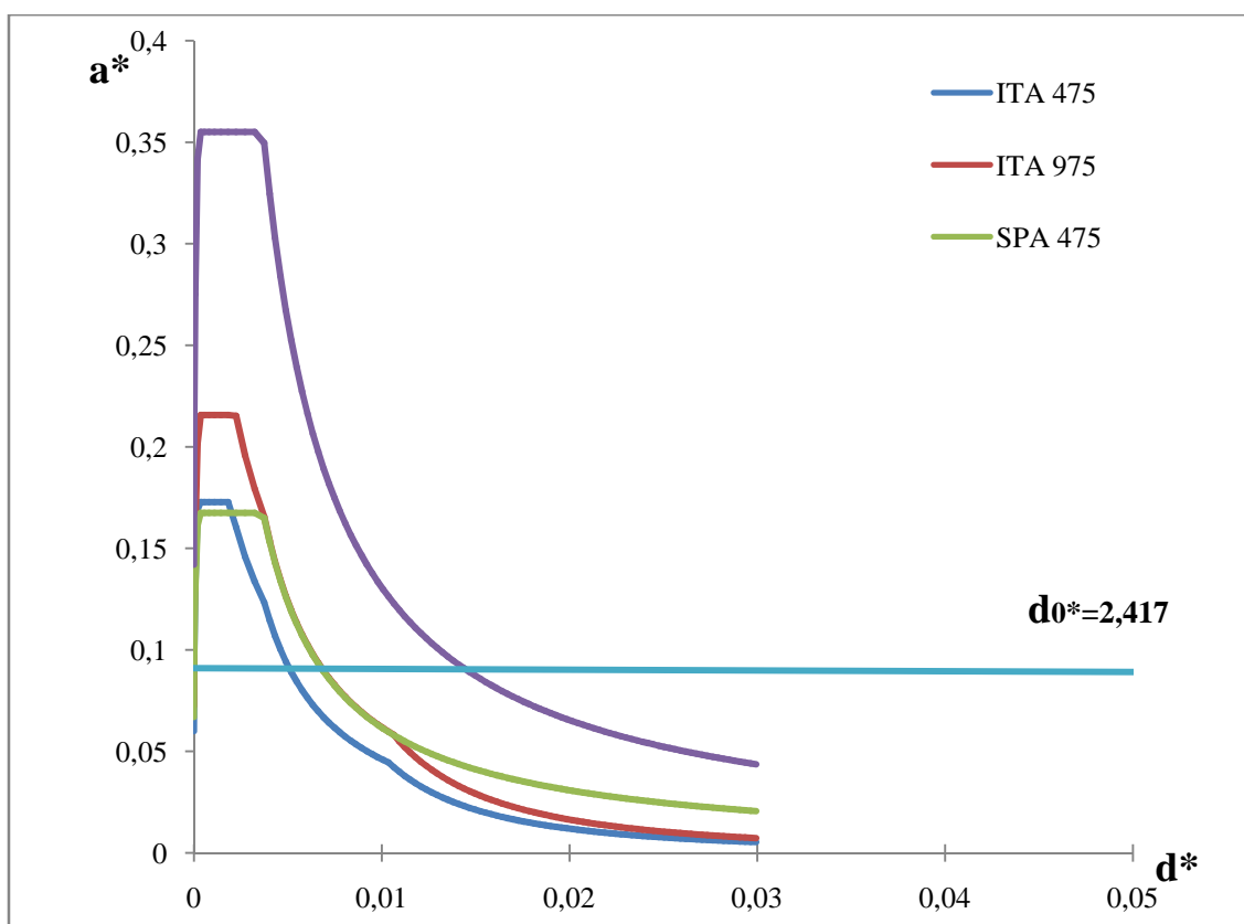
Figure A.21 – Capacity curve and demand spectrums of mechanism 8.
