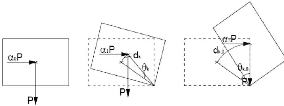
Figure 2.5 – Rotation \theta_{k,0} and displacement d_{k,0}
