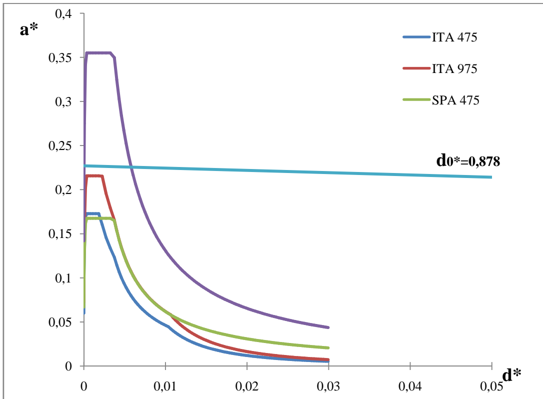
Figure A.15 – Capacity curve and demand spectrums of mechanism 5.
