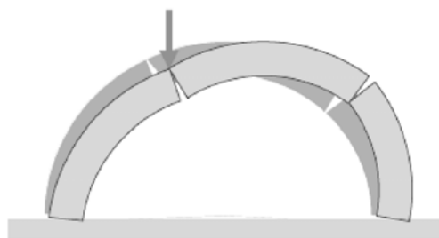
Figure 2.2 – Kinematic mechanism of an arch
