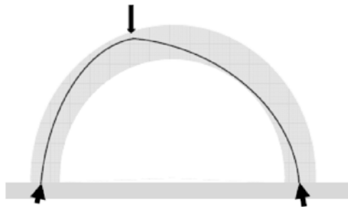
Figure 2.1 - Thrust line within a masonry structure
