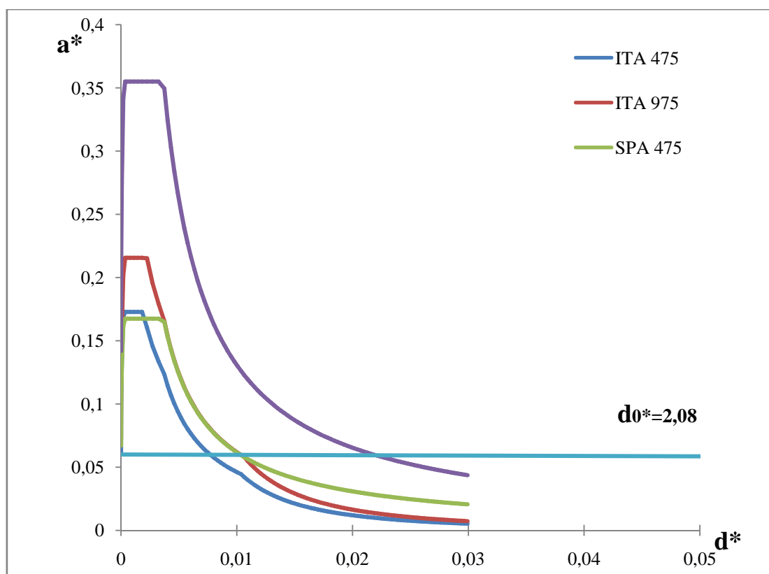
Figure A.17 – Capacity curve and demand spectrums of mechanism 6.
