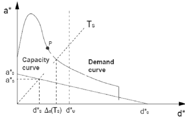
Figure 2.7 – Secant period T_s
