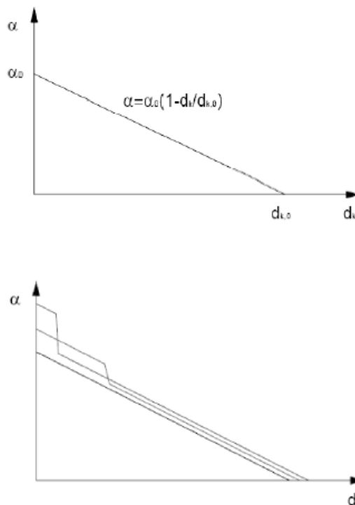
Figure 2.6 – Capacity curve
