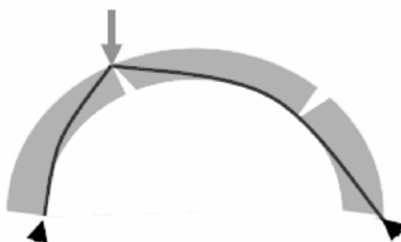
Figure 2.3 – Collapse mechanism of an arch
