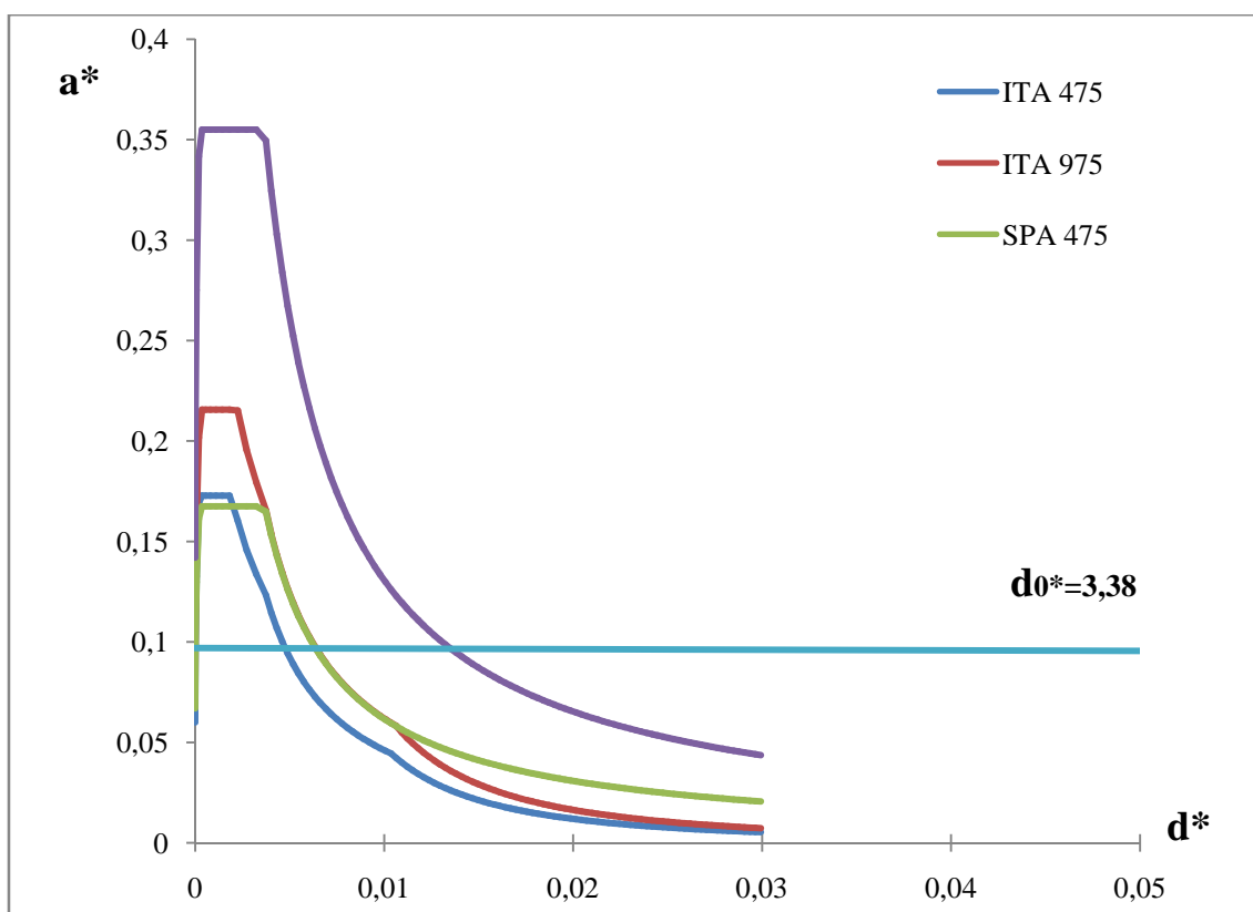
Figure A.9 – Capacity curve and demand spectrums of mechanism 2.
