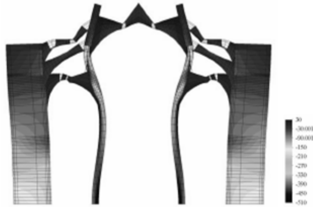
Stresses of the generalized matrix formulation model corresponding to a gravity load factor of 1.7 and neglecting the upper battery of flying arches (Salas (2002)).
