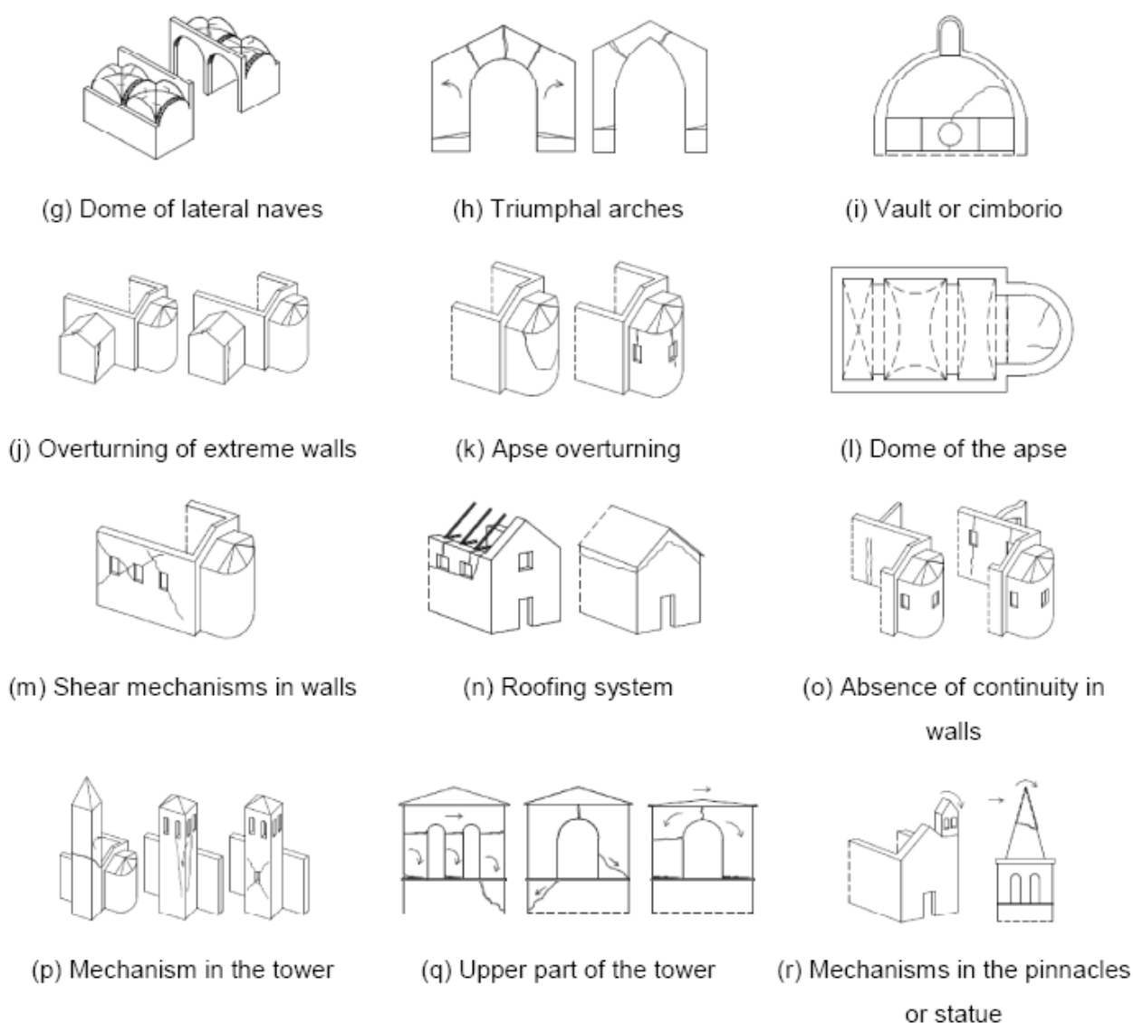
Figure 2.4 – Macroelements for churches proposed by Lagomarsino(1998)
