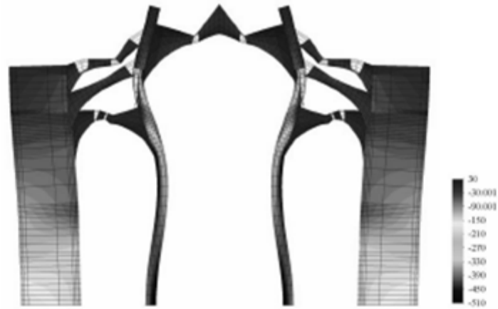
Collapse mechanism of the generalized matrix formulation model corresponding to a gravity load factor of 1.7 (Salas (2002)).
