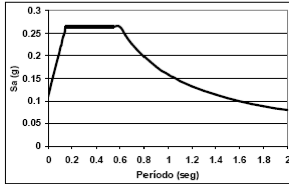
Spectral acceleration spectrum considering the deterministic scenario (Martinez (2007)).
