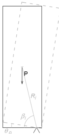
Figure A.4 – Parameters for calculation of the finite rotation \theta
