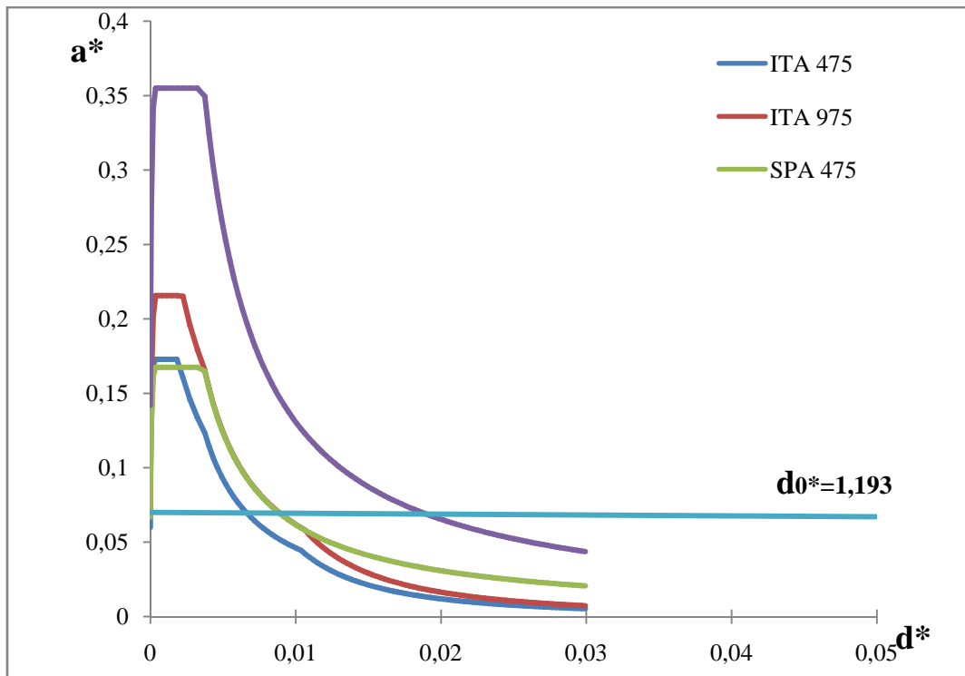
Figure A.11 – Capacity curve and demand spectrums of mechanism 3.
