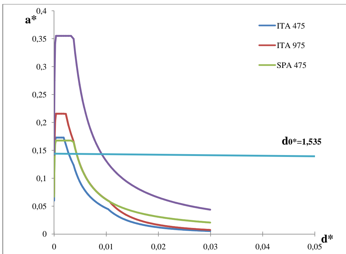
Figure A.25 – Capacity curve and demand spectrums of mechanism 10.
