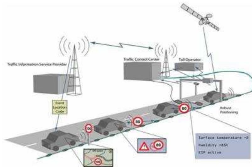
Fig. 1.9.1 Diagrama general de COOPERS
