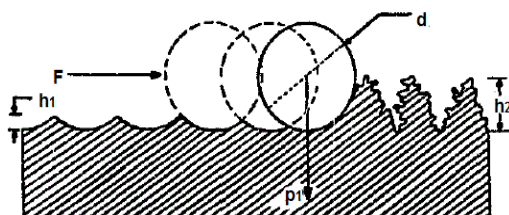
Figure 1. Burnishing schematically representation [2].
