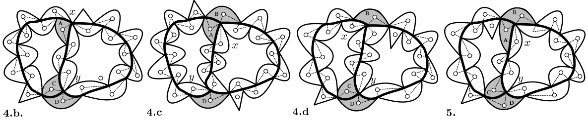
Figure 9: If F contains the edges of the stressed cycle then the graph H_F is the one formed by the dotted vertices and the white vertices.
