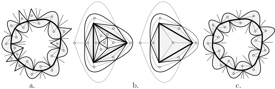
Figure 5: a) An example of the proof of Lema B.5. b) Examples of the case |C| = 3 of the proof of Lemma B.6. c) Example of the first case of the proof of Lemma B.6.
