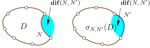
Figure 10: An example of the application of the function dif .
