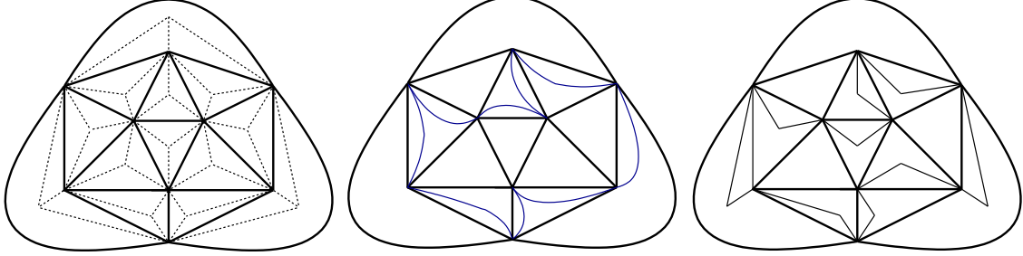
Figure 1: An example of a \Sigma -plane graph G drawn i) with its radial R_G ii) with a noose S that is not a cycle of R_G and with a noose S' that is a cycle of R_G and a vibration of S .
