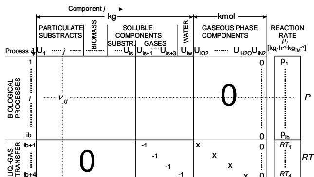
Fig. 2. Structure of the Petersen matrix, the vector of biological reaction rates (P) and the vector of liquid-gas transfer rates (RT), coupled into the reaction rates vector p .
