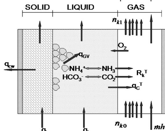
Fig. 1. The three phases in an elemental volume unit. Arrows indicate main fluxes direction.
