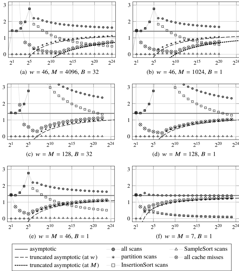
Figure 8 Comparison of cache miss counts ( \otimes ) from our idealized fully-associative LRU cache with different cache and block sizes M resp. B with corresponding scanned element counts ( \bullet ). The latter are also given separately for PARTITION ( * ), INSERTIONSORT ( \square ) and SAMPLESORT ( \triangle ). To make the counts comparable, the number of cache misses has been multiplied by B . All plots are normalized by n \ln n and show results for YQS_t^w with t = (1, 1, 1) and different Insertionsort thresholds w . The fat line (—) shows the leading-term asymptotic for scanned elements from Theorem 4.1, namely \frac{80}{57} n \ln n . The dashed line (- - -) is the truncated term \frac{80}{57} n \ln(\frac{n}{w}) and the dotted line (.....) shows \frac{80}{57} n \ln(\frac{n}{M}) , which is the leading term truncated at subproblems that fit into the cache.
