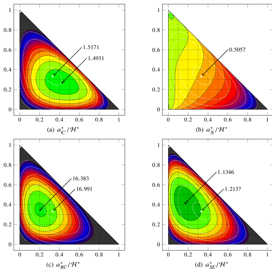
Figure 10 Contour plots for the limits of the leading-term coefficient of the overall number of comparisons, swaps, executed Bytecode instructions and scanned elements, as functions of \tau . \tau_1 and \tau_2 are given on x - and y -axis, respectively, which determine \tau_3 as 1 - \tau_1 - \tau_2 . Black dots mark global minima, white dots show the center point \tau_1 = \tau_2 = \tau_3 = \frac{1}{3} . (For swaps no minimum is attained in the open simplex, see main text). Black dashed lines are level lines connecting “equi-cost-ant” points, i.e., points of equal costs. White dotted lines mark points of equal entropy \mathcal{H}^* .
