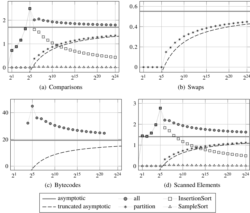
Figure 6 Comparison, swap, Bytecode and scanned element counts (●) normalized by n \ln n , for YQS_t^w with \mathbf{t} = (1, 1, 1) and w = 46 against the leading-term asymptotic \frac{a}{H} n \ln(n) (—) from Theorem 4.1 and its truncated version \frac{a}{H} n \ln(\frac{n}{w}) (- - -). For comparisons and scanned elements, the contributions from PARTITION (*), INSERTIONSORT (□) and SAMPLESORT (△) are also given separately. Note that swaps only occur during partitioning (Insertionsort uses single write accesses). For reasonably large n , the main contribution indeed comes from PARTITION, however, INSERTIONSORT on short subarrays also contributes significantly. This is probably true for all cost measures, even though not shown here in detail.
