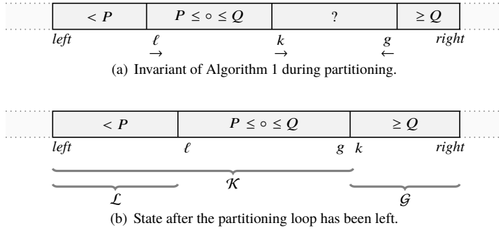
Figure 1 The state of the array \mathbf{A} during and after partitioning. Note that the last values attained by k , g and \ell are not used to access the array \mathbf{A} , so the positions of the indices after partitioning are by definition not contained in the corresponding position sets.
