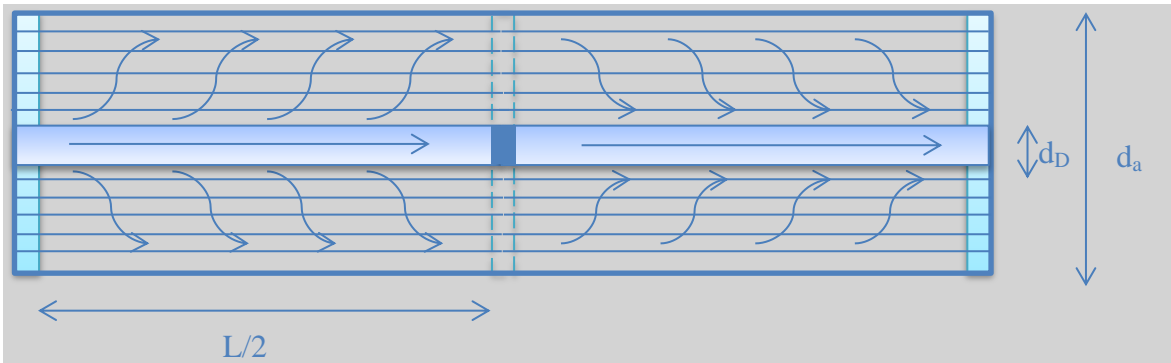
Figure 3. The schematic view of the cross flow hollow fiber module with the velocity profile of flow in the shell side compartment
