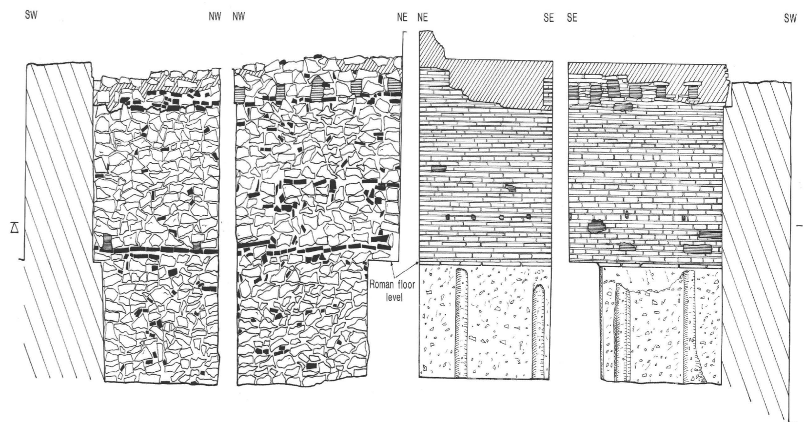
CASTELPORZIANO, Interior elevations of medieval tower, VICUS Building A, 47
