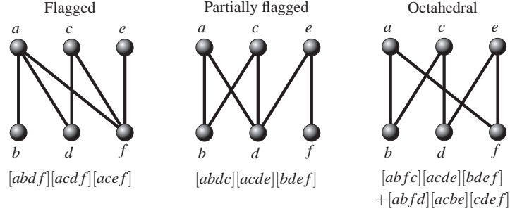
Fig. 2 The three possible topologies for 3-3 Stewart-Gough platforms –flagged, partially flagged and octahedral– and their corresponding pure conditions.
