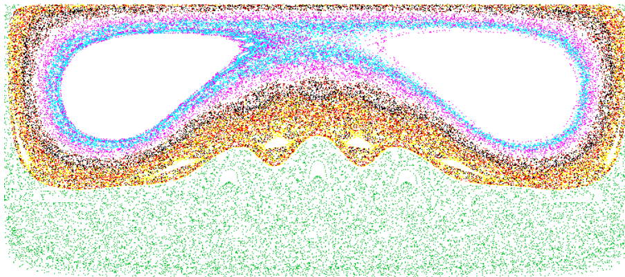
FIGURE 5. Poincaré map for the velocity field v_f or in other words the template, for K = 11 . This shows the underlying barriers (ie. the KAM tori) and the partial barriers (cantori) in the estuary's flow.
