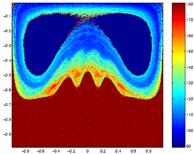
(b.) Exit times, n , for X = 0 and R = 0.01 , focusing in particular on the structure in regions 3 and 4, (see figure 7), by only considering and coloring values of 90 < n < 180 .
