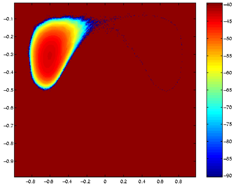
(b.) Exit times, n , for X = 0 and R = 0.01 , focusing in particular on the structure in regions of negative Stokes drift 1A and 2A , (see figure 7), by only considering values of -90 < n < -40 .
