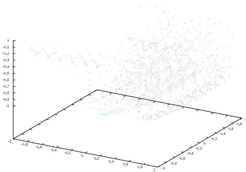
FIGURE 9. The Poincaré map in the full XYZ space, R = 0.01 , with different colours representing different initial conditions. Note for R \neq 0 trajectories stay within the confines of the estuary for much shorter time periods.
