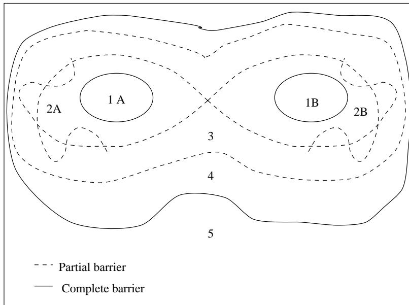
FIGURE 7. This shows the main regions we split the YZ space into. Regions 1A and 1B are bounded by the KAM curves surrounding the elliptical fixed points. The barrier separating regions 2A and 3 and regions 2B and 3 is that formed by the unstable and stable manifolds of the hyperbolic fixed point. While the barrier separating regions 3 and 4 is that formed by period 21 approximation to the cantor. The barrier separating regions 4 and 5 is a KAM curve. The outer bounds to region 5 are the boundaries of the estuary.
