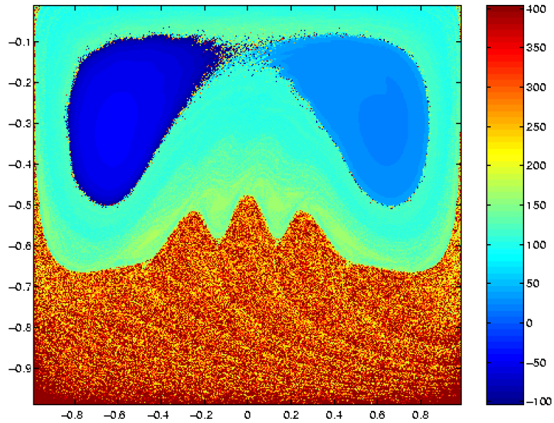
(a.) Exit times, n , for X = 0 and R = 0.01 , seen in projection in YZ space, and color contoured in n . Negative values of n correspond to regions of negative Stokes drift. All positive values of n greater than 400 are colored brown.
