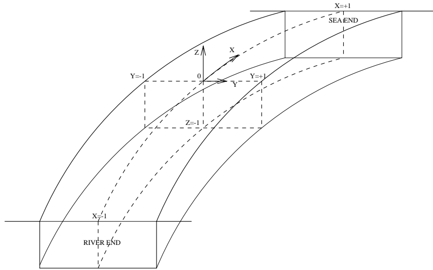
FIGURE 4. The bounds of our estuary.
