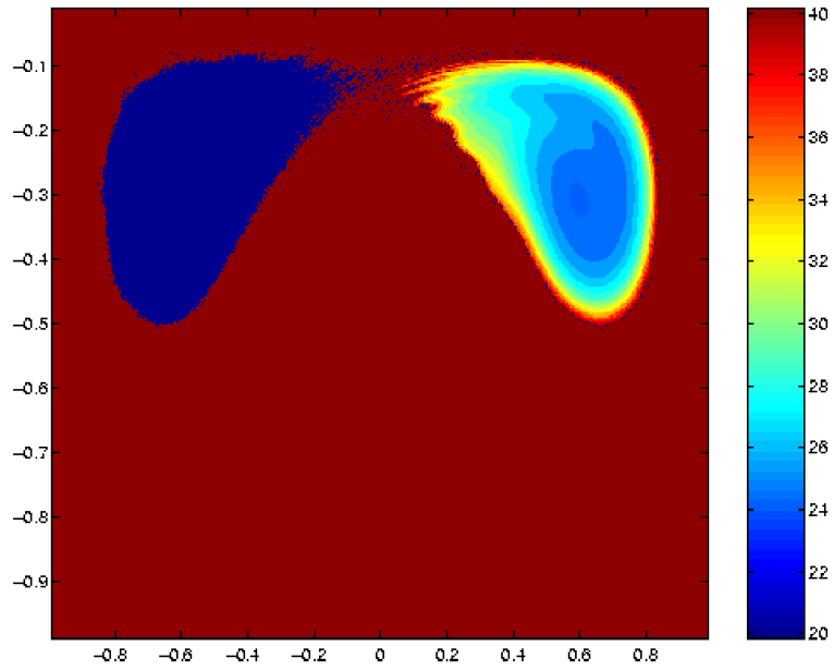
(a.) Exit times, n , for X = 0 and R = 0.01 , focusing in particular on the structure in regions 1B and 2B , (see figure 7), by only considering values of 20 < n < 40 .
