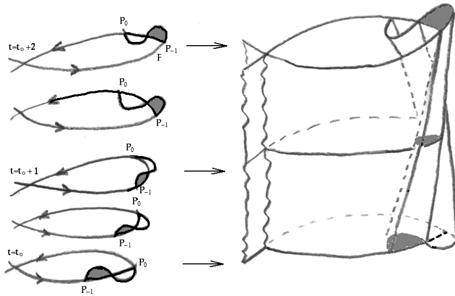
FIGURE 11. The turnstile lobe and the partial barrier, as viewed in the flow for one tidal period, (t_0 to t_0 + 2) , with P_0 being the primary intersection point, at time t_0 and P_{-1} being the pre-image of P_0
