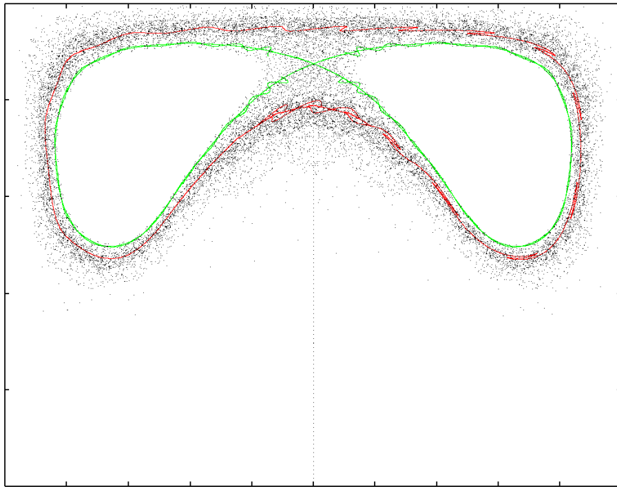
FIGURE 6. Turnstile lobes generated from a period 21 approximation to the two cantori (ie. seen as bounds to the dark band, in which there is a higher concentration of points) and also the unstable and stable manifolds of a hyperbolic fixed point, K = 11 .
