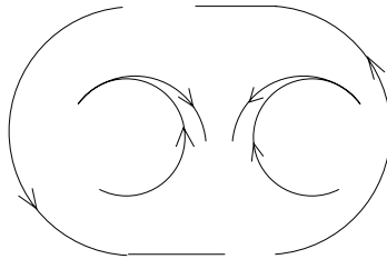
FIGURE 3. The stretching and folding via the large scale global circulations.
