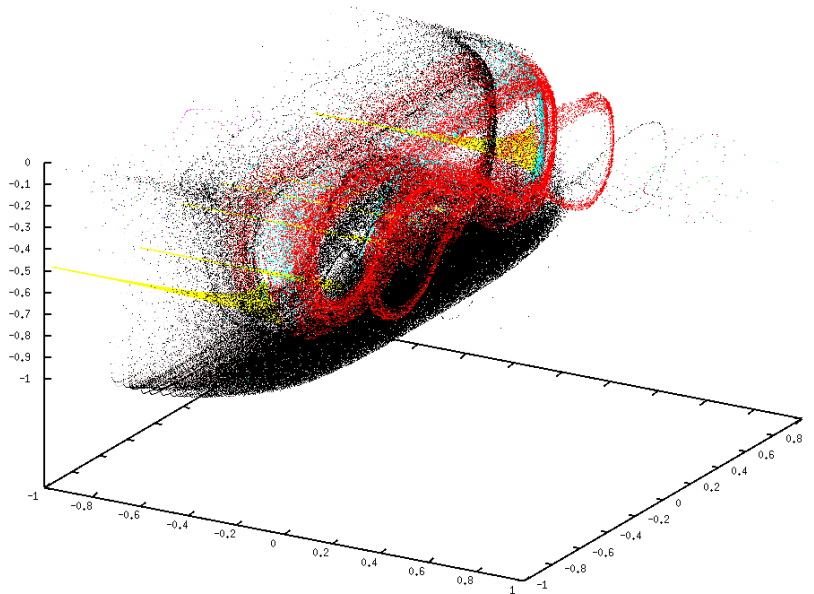
FIGURE 8. The Poincaré map in the full XYZ space, R = 0 , with different colours representing different orbits. This shows Stokes drift. An example of negative Stokes drift would be the yellow trajectory, while an example of positive Stokes drift would be the red trajectory
