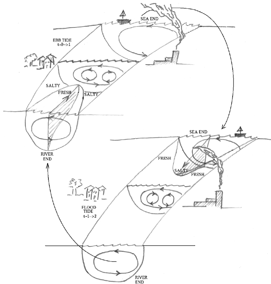
FIGURE 1. Cartoon of flow in an estuary, showing the single cell (wind or bend-driven) and the periodic two cell (density driven) transverse motion.
