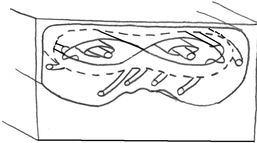
FIGURE 10. Tubes formed as a result of the evolution of the partial and complete barriers observed in the YZ map.
