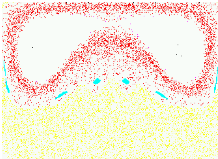
(a) YZ Poincaré map, t_0 = 0 .
