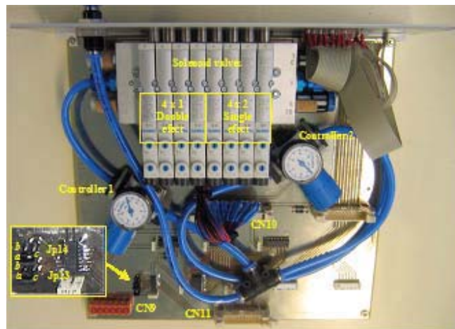
Fig. 7 Photograph representing the output card of the solenoid valves
