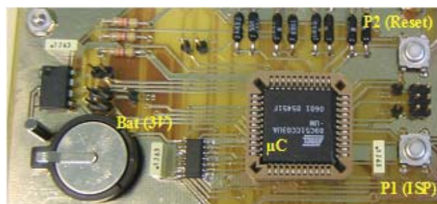
Fig. 5 Partial photograph showing the microcontroller subsystem
