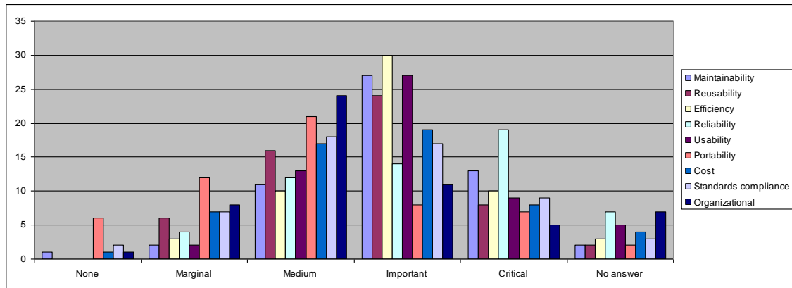
Fig. 1: importance of different types of NFR in software projects
