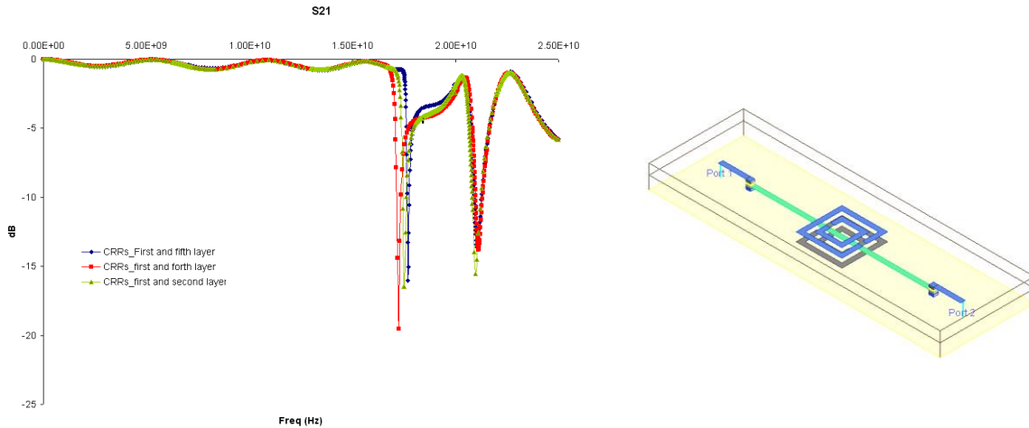
Fig. 5: Electromagnetic simulation insertion losses for two CSRR located in different layers.
