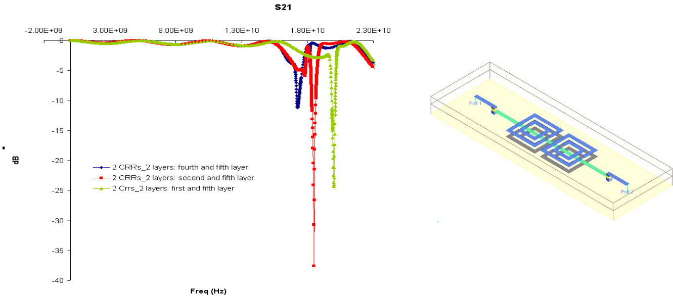
Fig. 7: Electromagnetic simulation insertion losses for two CSRRs stage combined in two LTCC layers.
