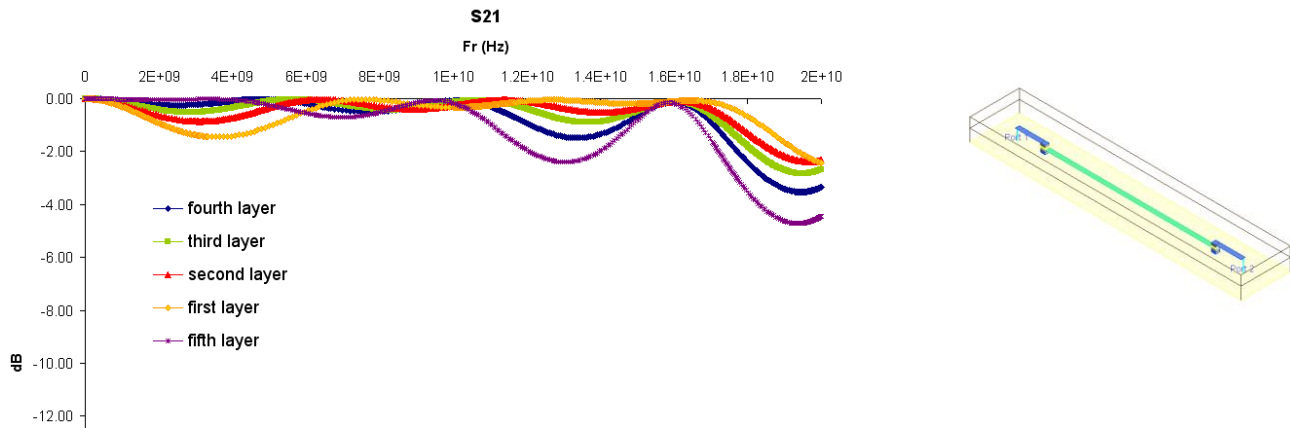
Fig. 3: Electromagnetic simulation of the insertion losses of the considered stripline with regard to the layer position in the z-plane.
