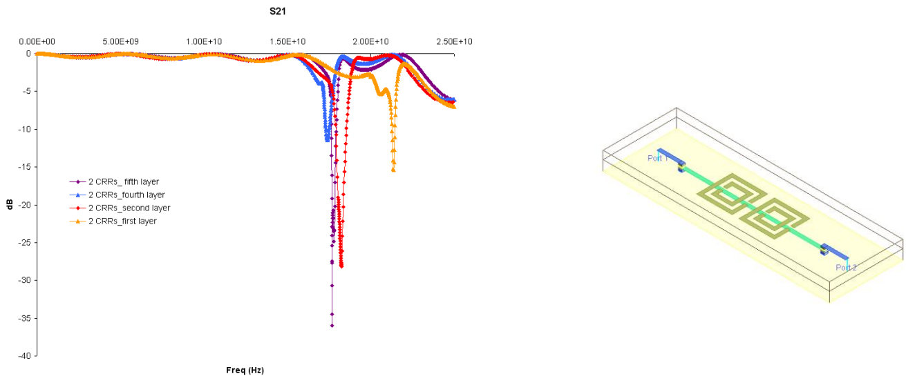
Fig. 6: Electromagnetic simulation insertion losses for two CSRRs located in the same layer.
