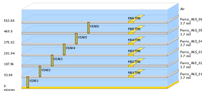
Fig. 1: Cross section of the 6 metal layer LTCC technology
