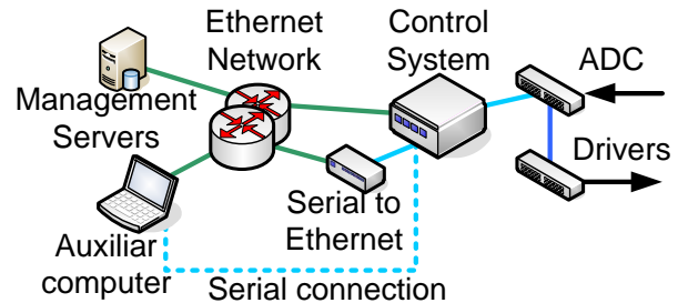
Figure 2 Diagram of the subsea control system
