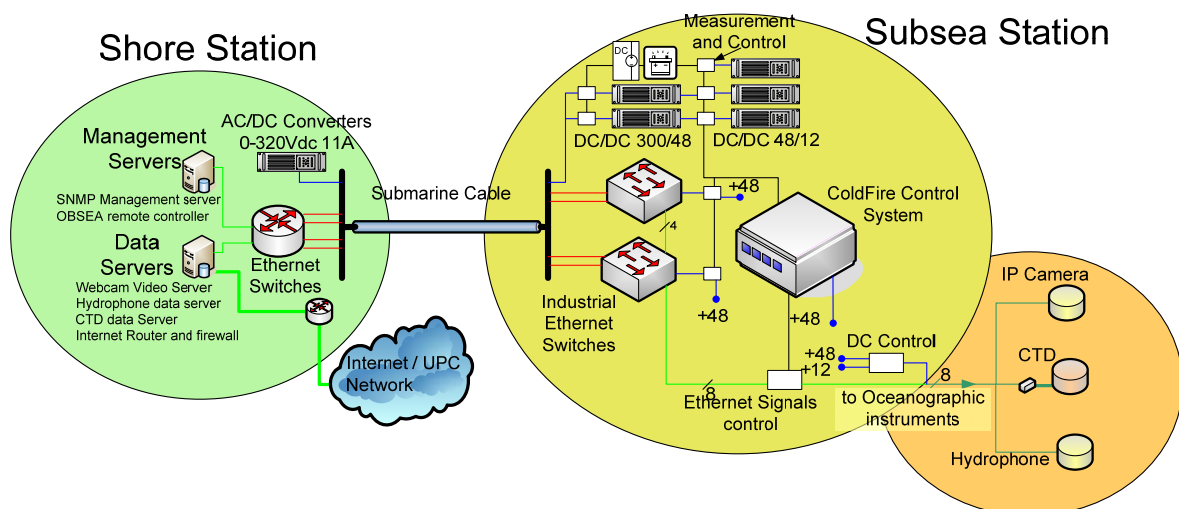
Figure 1 General diagram
