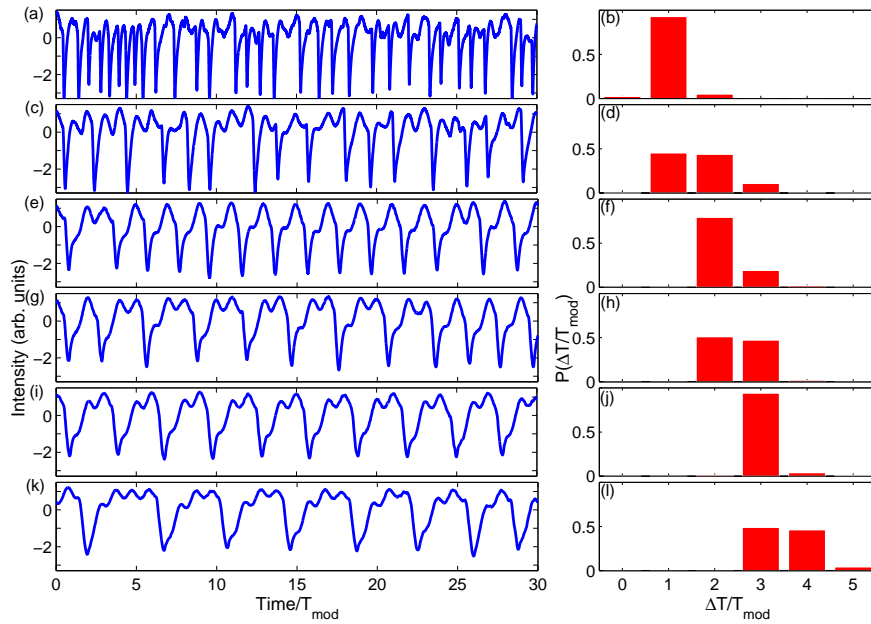
Fig. 1. Experimental time series of LFF intensity spikes (left column) and the corresponding inter-spike-interval (ISI) distribution (right column). The modulation amplitude is 1.2% of I_{DC} and the modulation frequency is 7 MHz (a-b); 14 MHz (c-d); 26 MHz (e-f); 31 MHz (g-h); 39 MHz (i-j); 49 MHz (k-l). In the left panels only 30 modulation cycles are shown, but the ISI distributions in the right panels are computed from 40000 ISIs.
