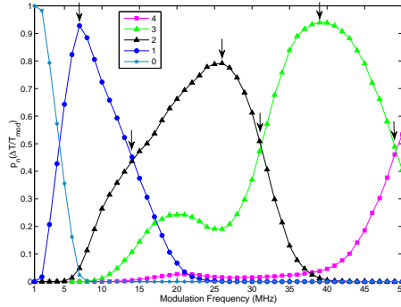
Fig. 3. Probability, p_n , that an ISI value is with the interval nT_{mod} - T_{mod}/2, nT_{mod} + T_{mod}/2 . n values in the legend. The first five probabilities are shown, for the same modulation amplitude as Fig. 1 (1.2%).
