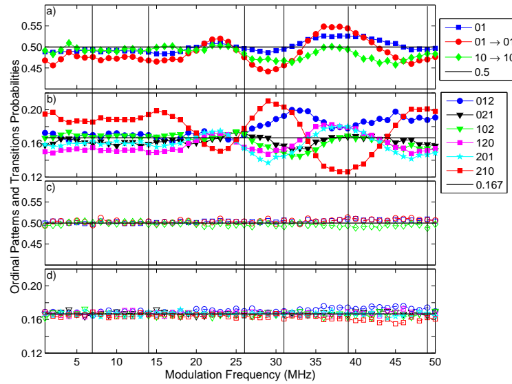
Fig. 4. (a) Probabilities of D = 2 ordinal patterns and the transition probabilities. (b) D = 3 OPs probabilities. (c), (d) Same as (a),(b) but when the OPs and TPs are computed from surrogate (shuffled) IDI sequences.
