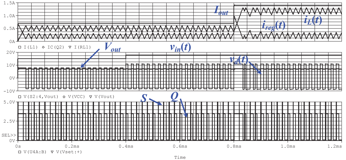
Fig. 5. Transient response of the constant-frequency linear-assisted converter with V_{in}=15\text{ V} . It can be seen the response of the circuit to an input step from 15 V to 18 V in the time instant t=400\ \mu\text{s} , and when there is a decrement of the load resistance from 10 \Omega to 5 \Omega in t=800\ \mu\text{s} .
