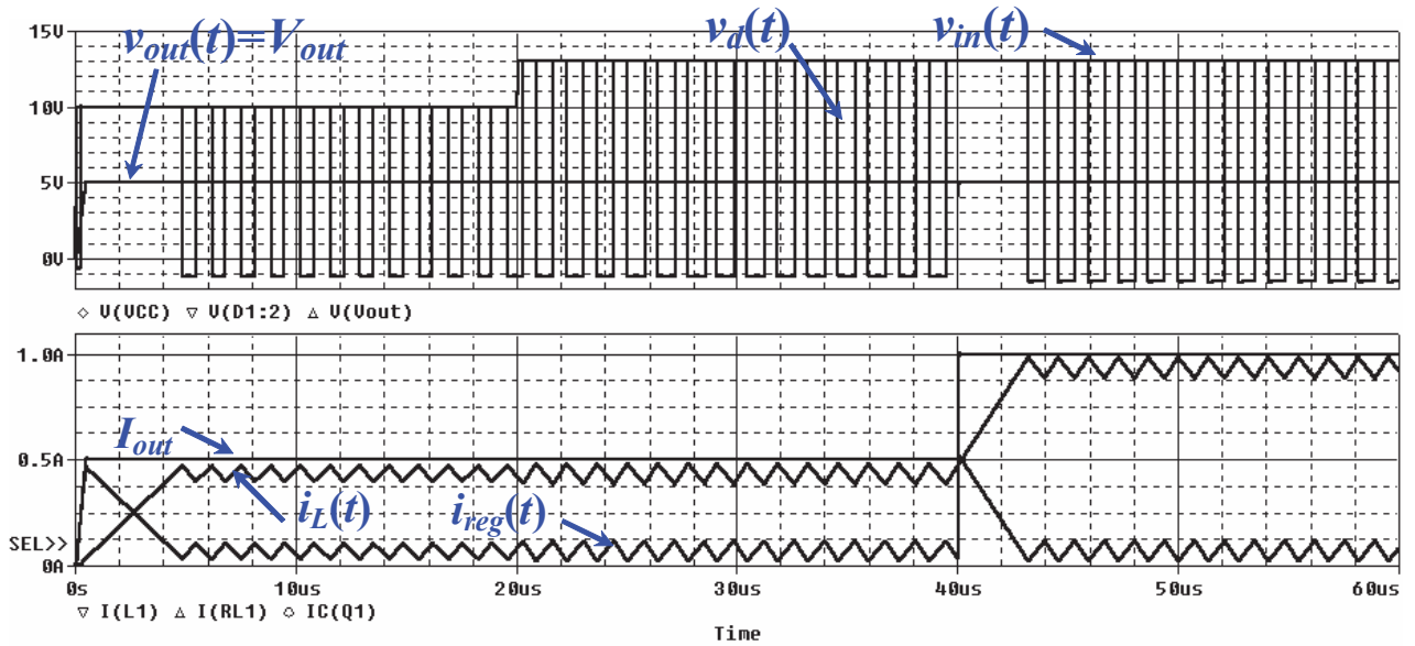
Fig. 3. Transient response of the variable-frequency linear-assisted converter with V_{in}=10 V . It can be seen the response of the circuit to an input step from 10 V to 13 V in the time instant t=20 \mu s , and when there is a decrement of the load resistance from 10 \Omega to 5 \Omega in t=40 \mu s .
