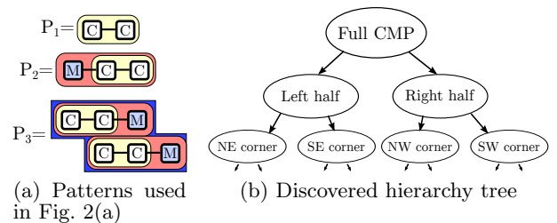
Figure 3: List of patterns and hierarchy tree.
