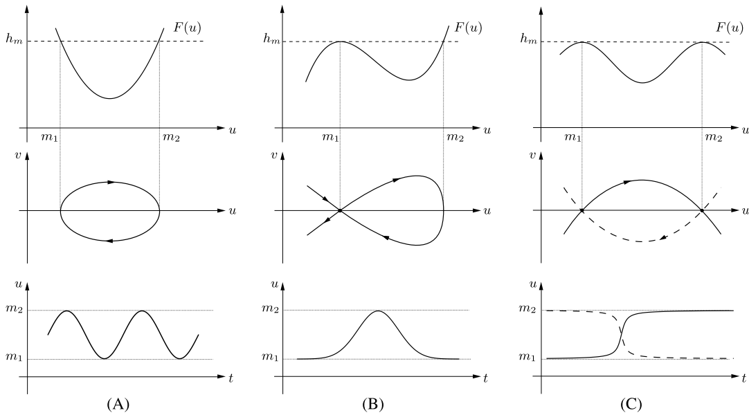
Fig. 1. Global strong TWS of (1). (A) Periodic wave; (B) Solitary wave or pulse; (C) Smooth front.
