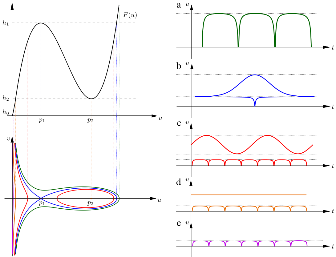
Fig. 5. Singular TWS of Eq. (15) varying the energy level h in the case 0 < p_1 < p_2 and h_2 > h_0 . (a) cusped periodic waves for h > h_1 ; (b) cusped and smooth solitary waves for h = h_1 ; (c) cusped and smooth periodic waves for h_1 > h > h_2 ; (d) cusped periodic waves and constant solutions for h = h_2 ; (e) cusped periodic waves for h_2 > h > h_0 .
