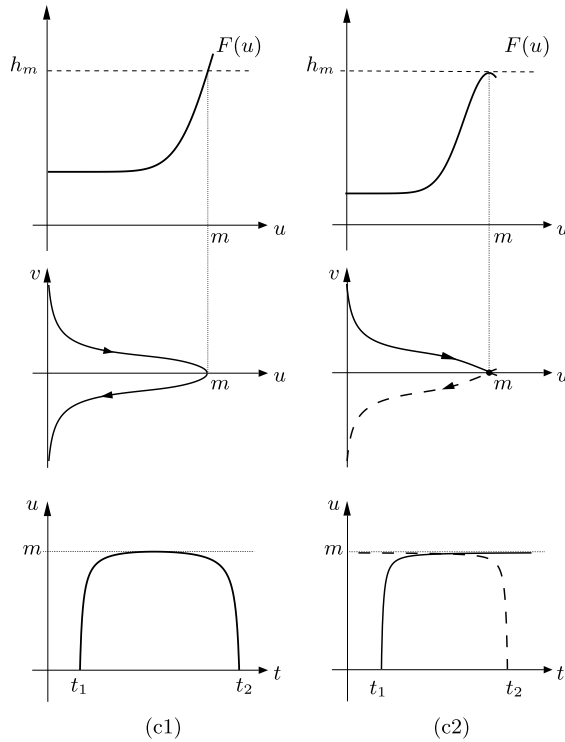
Fig. 4. Strong solutions of (1) defined in a subset of \mathbb{R} associated to curves \gamma_h with unbounded component v near the singular line \{u = 0\} \times \mathbb{R} . They provide elementary forms to construct TWS with cusps.
