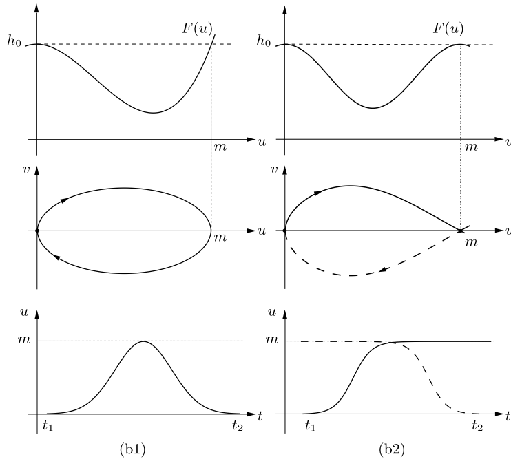
Fig. 3. Strong solutions of (1) defined in a subset of \mathbb{R} with energy h = h_0 when F'(0) = 0 . These provide elementary forms to construct TWS of class C^1(\mathbb{R}) (with compact support).
