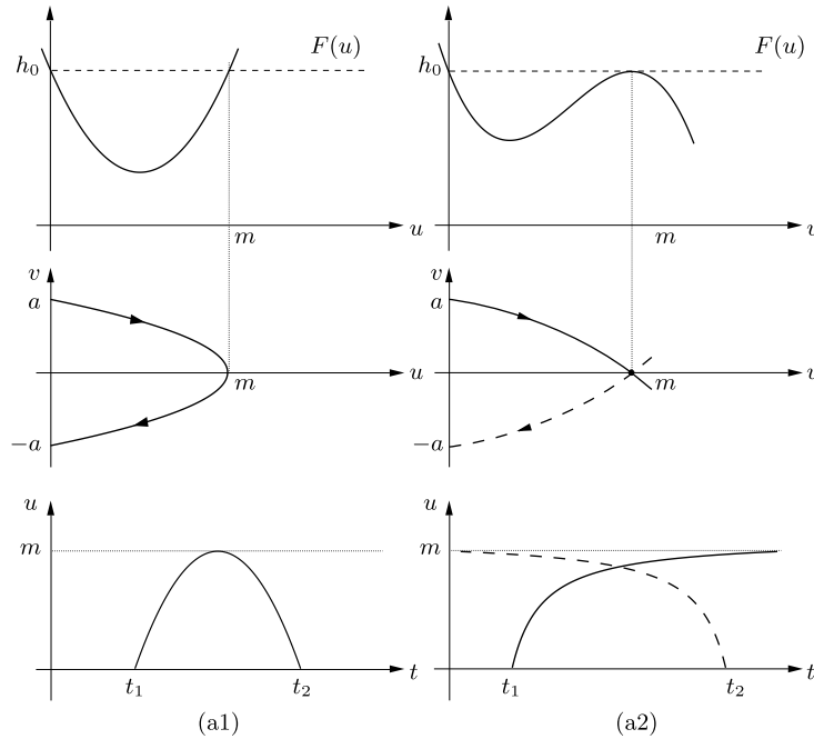
Fig. 2. Strong solutions of (1) defined in a subset of \mathbb{R} with energy h = h_0 when F'(0) \neq 0 . These provide the elementary forms to construct peaked periodic and solitary TWS.
