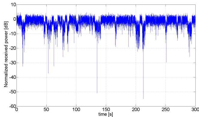
Fig. 14. Five minutes sample of the 30 minutes channel series (power in logarithmic scale) used in the simulations. The time series has been generated with a channel simulator implementing the LMS Perez-Fontan model in suburban environment, vehicle speed 50 kmph and satellite elevation 30^\circ .
