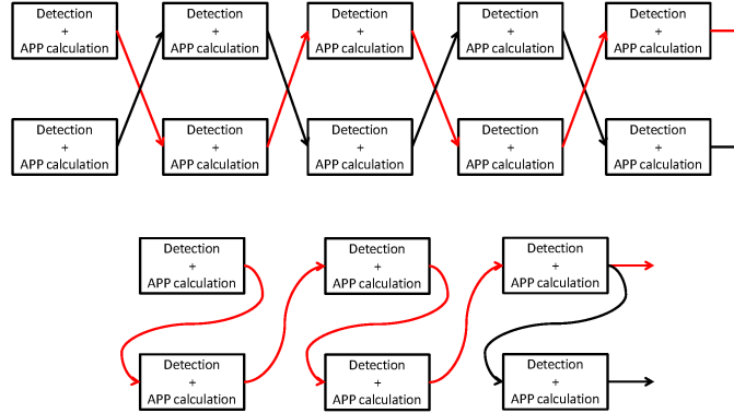
Fig. 6. Comparison between the proposed method and a parallel MUD scheme. In red we put into evidence the decoding path for the reference signal. In the figure we show only the propagation of the APPs. In the practical implementation of both schemes the detector takes as input also the received signal, not indicated for sake of clarity.
