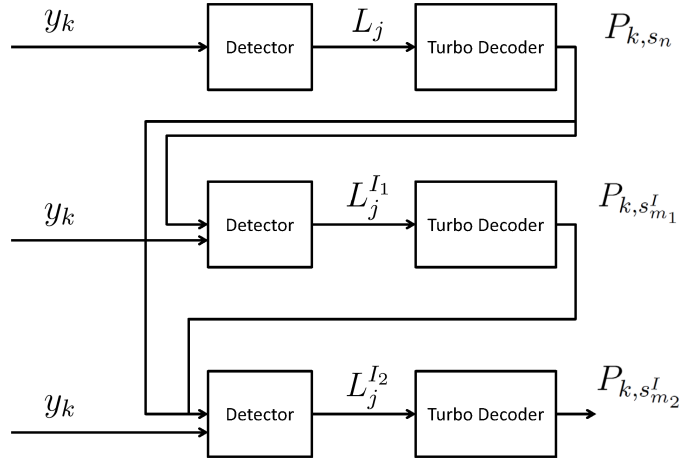
Fig. 3. Block diagram illustrating an iteration of the SISO detector/decoder.
