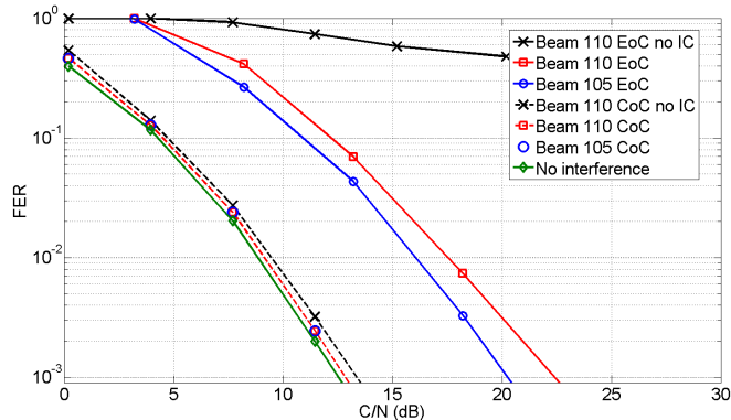
Fig. 15. Frame error rate for the reference signal using the simplified SIC scheme with one iteration (one detection and one decoding iteration). A 30 minutes LMS channel series in suburban environment generated according to [23] has been used. 10 interferers have been considered using the C/I values in Table I. Bearer F80T025Q1B-L8 (QPSK, channel code rate 1/3, symbol rate 8400 symbols per second) of standard [10] has been adopted for all signals.
