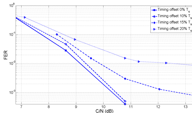
Fig. 16. FER in AWGN, simplified MUD, QPSK rate 1/3 used in all signals. Curves for different relative delays are shown. Delays are expressed in fraction of symbol duration T_s .
