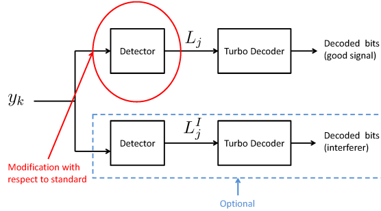
Fig. 9. Proposed simplified SIC scheme. Only the strongest interferer is taken into account and no iterative detection/decoding is applied (i.e., reference signal is detected as described in Section III and decoded using the turbo decoder specified in [10]). Optionally, also the strongest interfering signal can be decoded.
