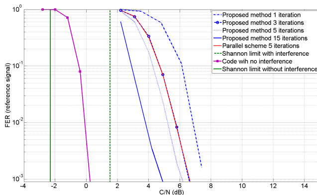
Fig. 5. FER in AWGN, QPSK rate 1/3 used in all signals. The Shannon limit for the case of no interference and for the case with one interferer with C/I = 0 dB are also shown. The FER for a scheme in which the signals are decoded in parallel rather than serially (as in the proposed scheme) is also shown. It can be seen how the loss of the proposed scheme with respect to the Shannon limit for a FER of 10^{-3} is only slightly larger than the loss due to the code (curves in case of no interference). It can be also seen how the parallel scheme requires more iterations with respect to the proposed scheme.
