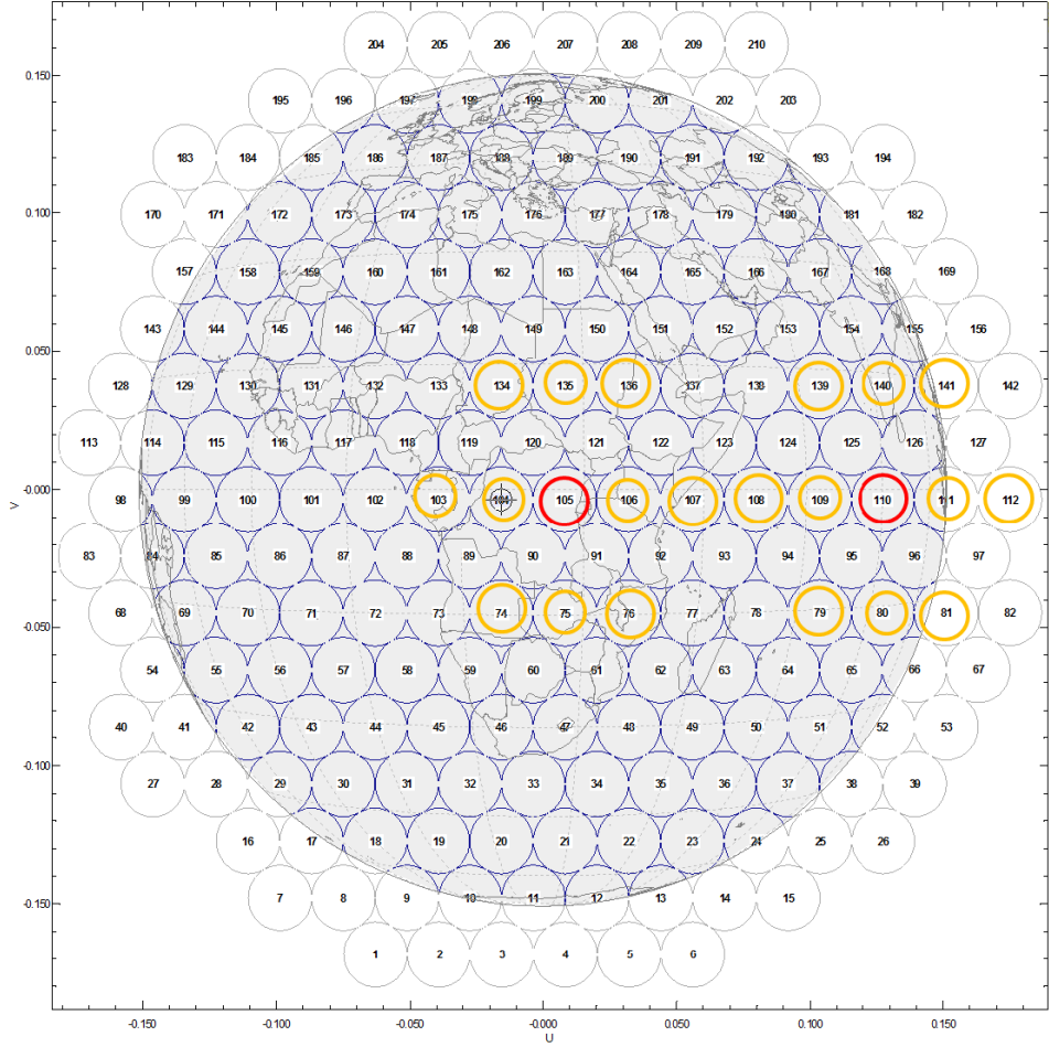
Fig. 1. Considered reference and interfering beams and conventional numbering. Reference and interfering beams are shown in red and yellow, respectively.
