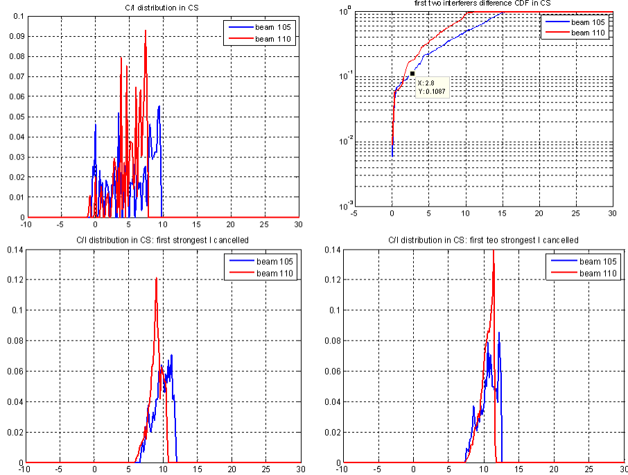
Fig. 8. Distribution of interference across the covered area in case: 1) all interferers are present (top-left), 2) the strongest interferer has been removed (bottom-left), 3) the two strongest interferers have been removed (bottom-right). The CDF of the difference between the two strongest interferers across the beam is also shown (top-right).
