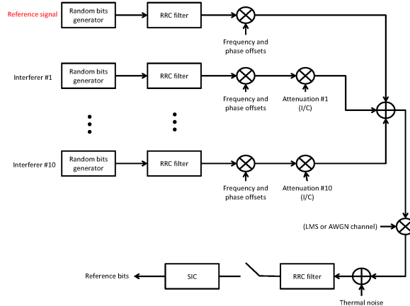
Fig. 10. Simulation setup in AWGN and LMS channels.
