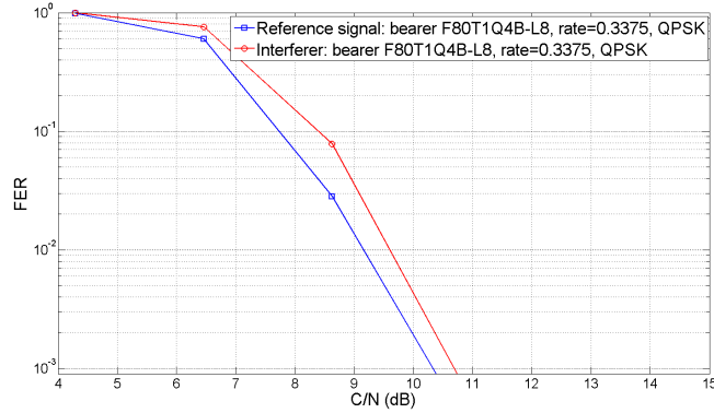
Fig. 11. FER in AWGN, simplified MUD. Bearer F80T1Q4B-L8 (QPSK rate 1/3, symbol rate 33600 sym/sec, roll-off 0.25) is used for all signals. The interference pattern for beam 110 EoB detailed in Table I (worst case scenario) has been used.
