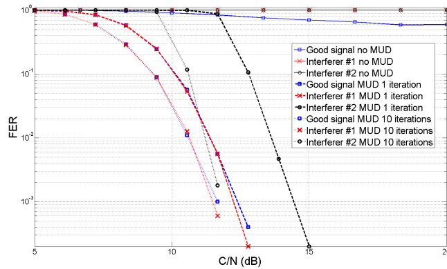
Fig. 4. FER curves for the reference signal and for two interferers. The interferers have a relative C/I of 0 and 6 dB, for a global C/I of -0.9732 dB. A bearer with QPSK modulation, rate 1/3 and 360 data bits per FEC codeword have been used for all signals.
