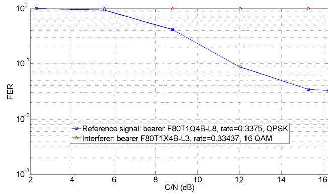
Fig. 13. FER in AWGN, simplified MUD. Bearer F80T1Q4B-L8 (QPSK rate 1/3, symbol rate 33600 sym/sec, roll-off 0.25) is used for the reference signal while bearer F80T1X4B-L3 (16 QAM rate 1/3, symbol rate 33600 symbols per second, roll-off 0.25) is used for the interferers. Note that rate 1/3 is the lowest code rate available in [10]). The interference pattern for beam 110 EoB detailed in Table I (worst case scenario) has been used.
