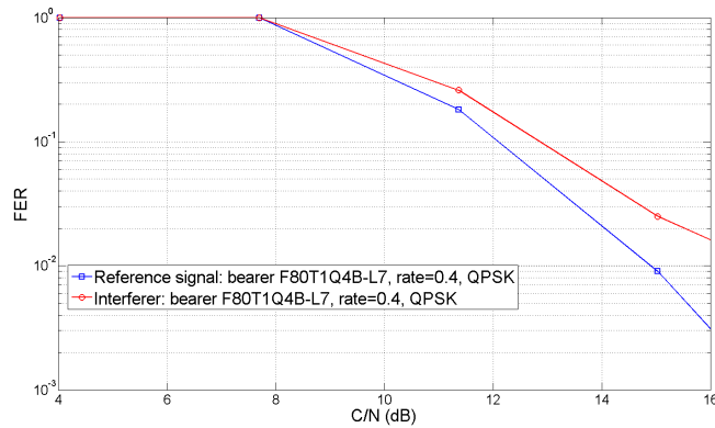
Fig. 12. FER in AWGN, simplified MUD. Bearer F80T1Q4B-L7 (QPSK rate 2/5, symbol rate 33600 sym/sec, roll-off 0.25) is used for all signals. The interference pattern for beam 110 EoB detailed in Table I (worst case scenario) has been used.
