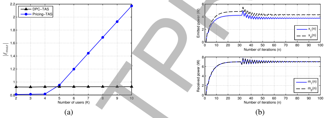
Figure 9: Inequality of Pricing-TAS: (a) Comparison of the maximum eigenvalue of the matrix (\mathbf{I} - \beta\mathbf{DA}) for DCP-TAS and the matrix \mathbf{B} for Pricing-TAS, and (b) Pricing-TAS ( \mu = -0.2 ) emitted and received power evolution when number of users increases from 4 to 5.
