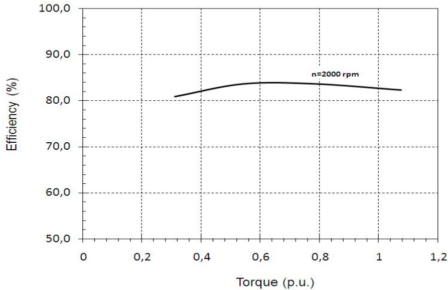
Fig. 6. Global efficiency vs. torque for the 8/6 SRM drive
