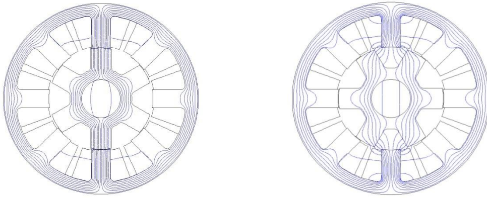
Fig. 2. Flux plots of the 8/6 SRM in aligned (left) and unaligned (right) positions obtained using the FLUX 2D FEM package
