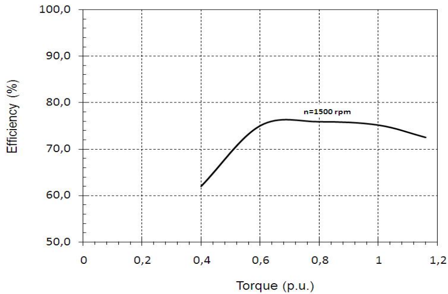
Fig. 4. Global efficiency vs. torque for the IM (Eff3) drive
