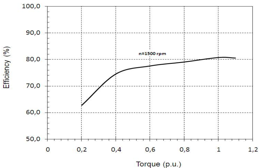
Fig. 5. Global efficiency vs. torque for the IM (Eff1) drive
