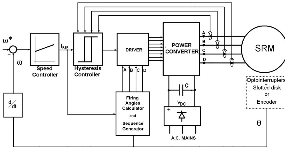
Fig. 3. Schematic diagram of the SRM drive
