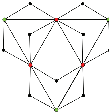
Figure 1: An example of \tau^2(G) . Red vertices denote the initial K_3 vertices while green and black vertices have been introduced to obtain \tau(K_3) and \tau^2(K_3) , respectively.
