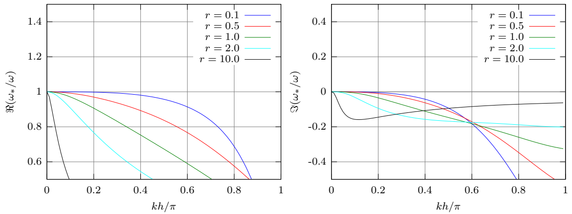
Figure 18: OSS + BDF2 for C_\tau = 0.2
