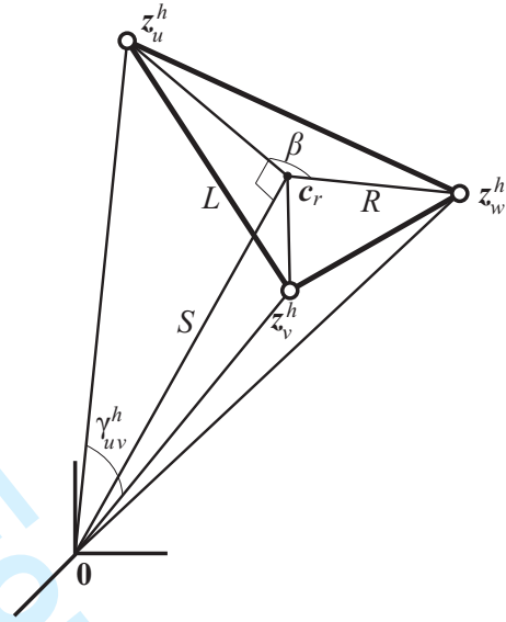
Figure 1: The projection of r = 3 vertices of a d -spread.
