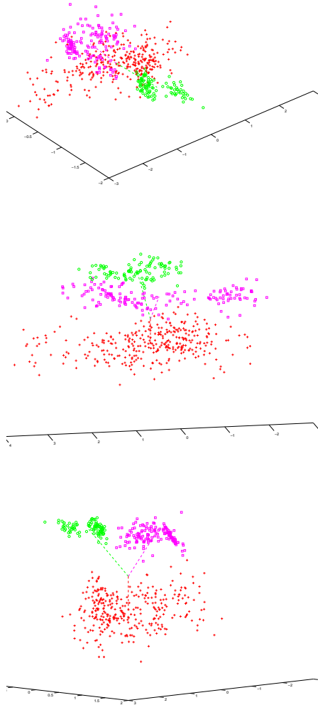
Figure 1: Three chosen illustrative MGT projections of the Italian Olive Oil data set, colour-labelled to show the main three classes ( South : red crosses, Sardinia : green circles and North : magenta squares), defined in three different GTM nodes. The bottom plot exemplifies a projection in which the three clusters are clearly separated, while the top and middle plots correspond to projections in which it is more difficult to visually disentangle the cluster structure.
