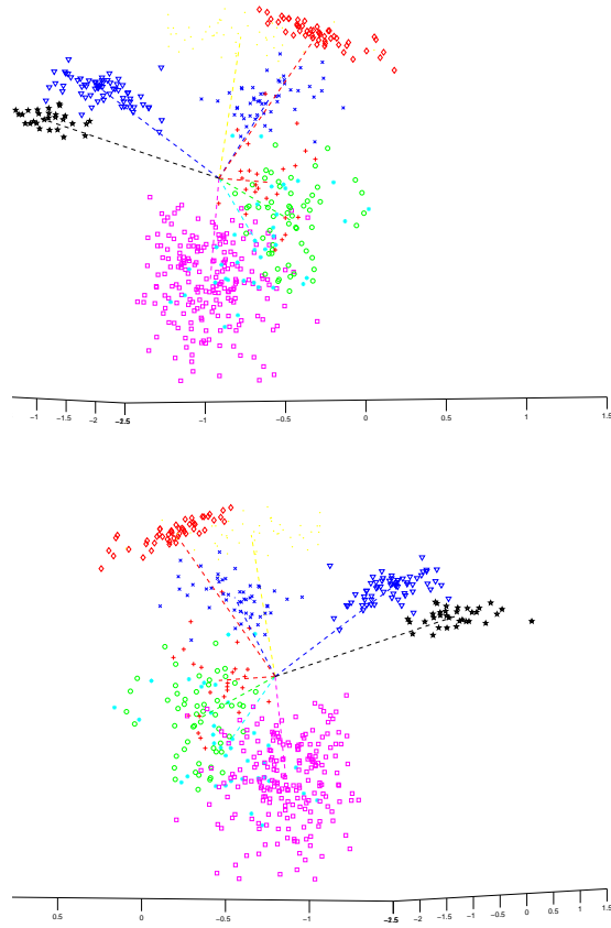
Figure 2: Two chosen illustrative MGT projections of the Italian Olive Oil data set, this time colour-labelled to show the detailed nine sub-class structure, defined in two different GTM nodes. The internal structure of Sardinian cluster is shown in two sub-clusters (black pentagrams and blue triangles)
