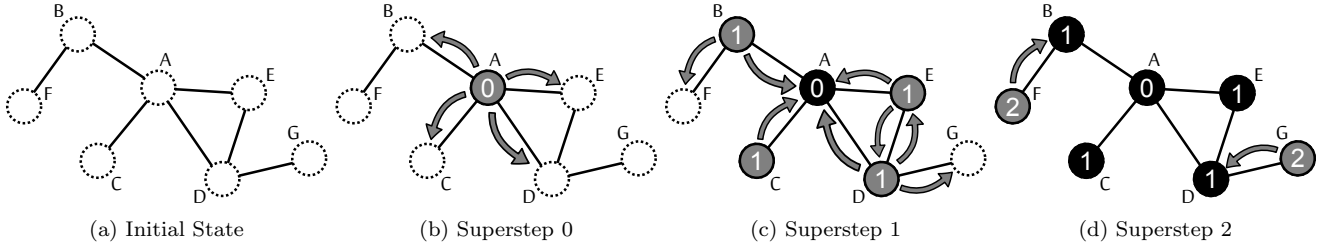
Figure 2: Computing the eccentricity of vertex A.
