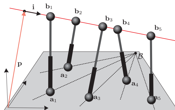
Fig. 1. A 5-DoF 5-SPU parallel manipulator with collinear attachments in the platform and coplanar in the base.
