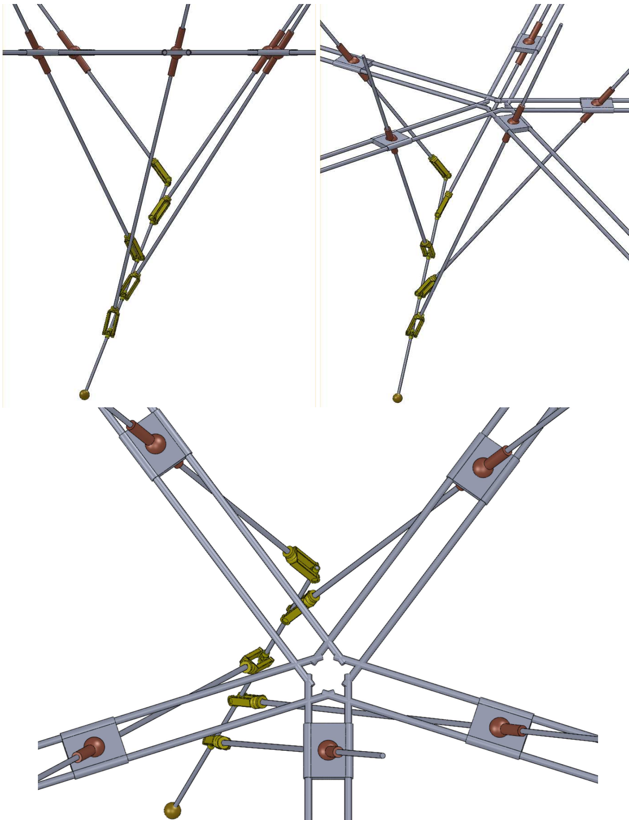
Fig. 3. Three different views of the proposed 5-DoF 5-SPU parallel platform in the same configuration. The base attachments can be independently moved along radial guides without altering the singularity locus of the platform.
