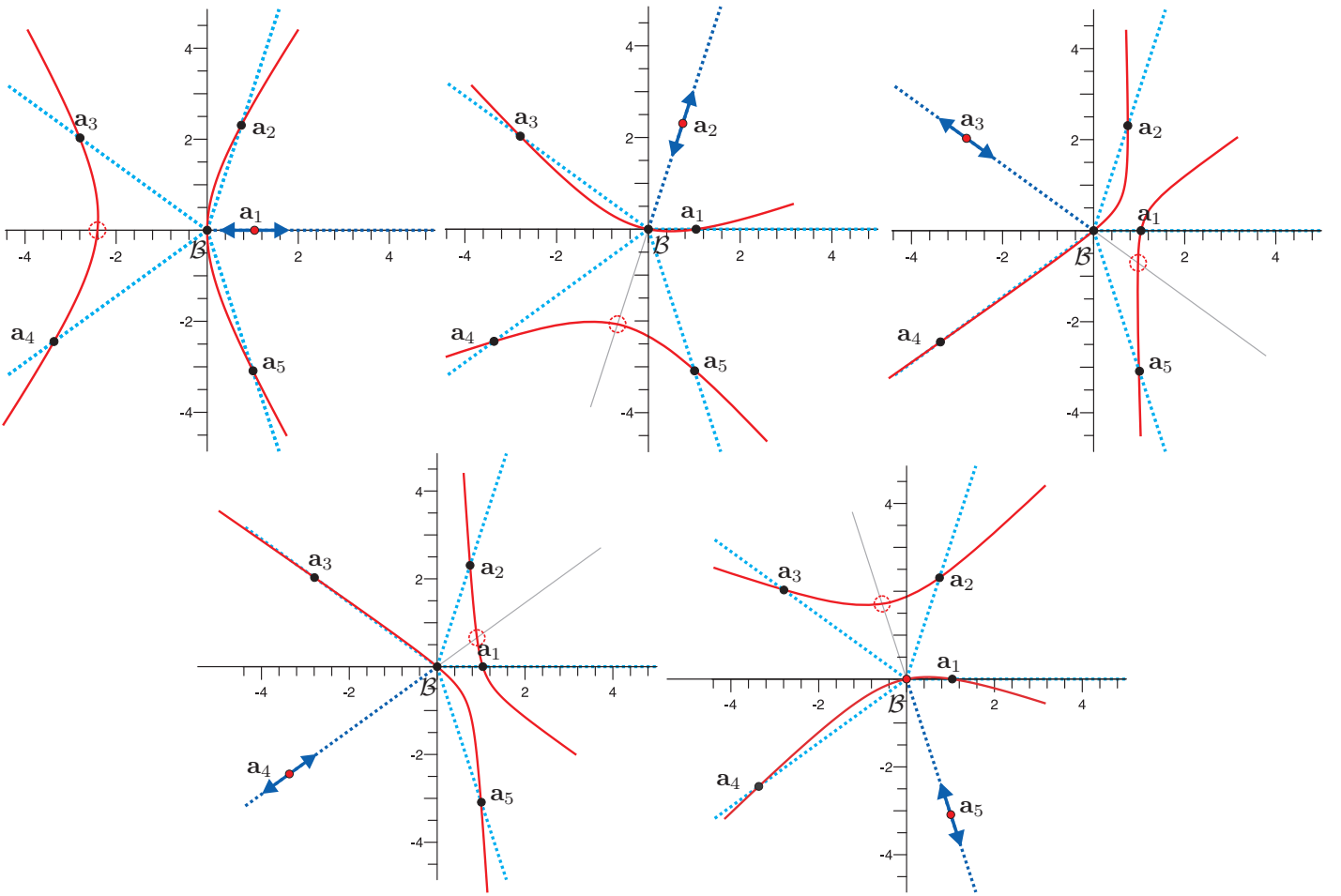
Fig. 4. The base attachments in the proposed architecture can be independently moved along radial guides (shown in dotted lines) without leading to architectural singularities because each attachment cannot be located on the conic (shown in solid lines) defined by the other four attachments and the origin. Moreover, no four attachments can be made collinear. If the attachments could move along their whole associated \mathcal{B} -lines, they could overpass the origin giving rise to the possibility of intersect the conic (shown in dotted circles) thus leading to architectural singularities. Limiting the possible reconfigurations to radial guides, this possibility is totally excluded.
