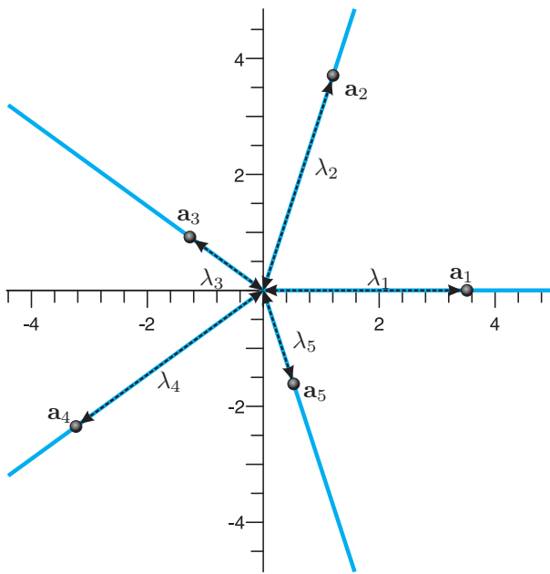
Fig. 6. The value of \det(\mathbf{T}) is multiplied by a constant that only depends on the distances of the attachments to the origin.
