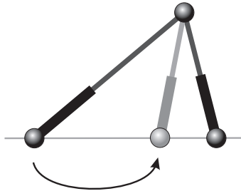
Fig. 2. When two legs in a Stewart-Gough platform share an attachment, the other two attachments can be reconfigured without altering the singularities of the platform.
