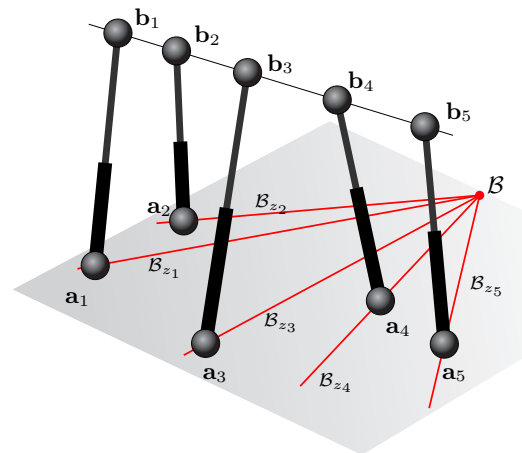
Fig. 4. The one-to-one correspondence between the attachments in the line and the lines of the pencil centered at B . Each value of z_i defines a point in the line, \mathbf{b}_i = \mathbf{p} + z_i \mathbf{i} , and a line in the plane B_{z_i} .
