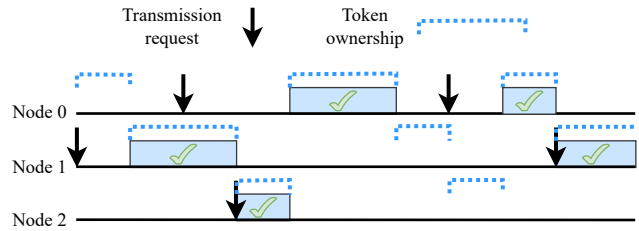
Figure 5: Timing diagram of the token passing protocol.
