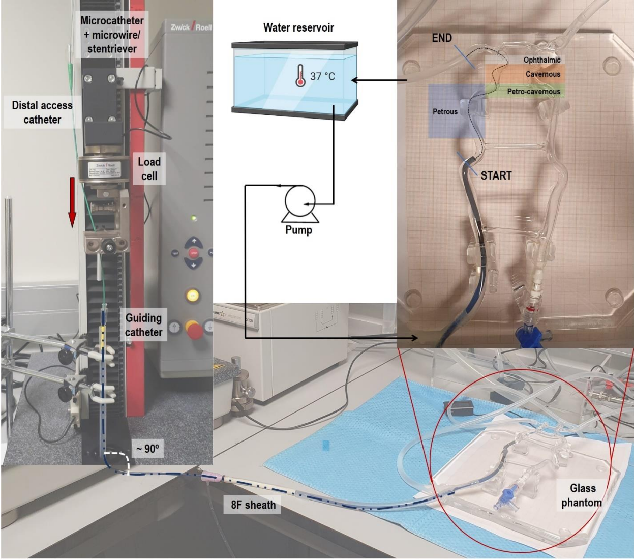
Figure 1. Experimental setup to monitor track forces of various navigation techniques and DACs.
