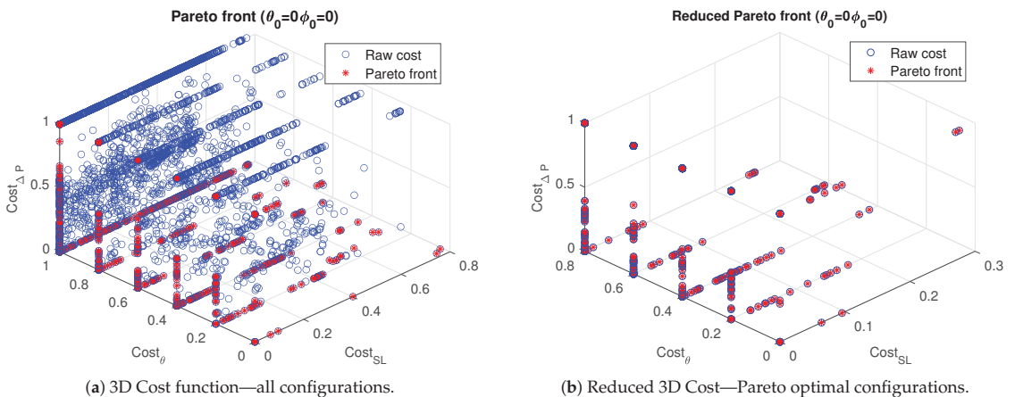
Figure 14. Optimization process.
