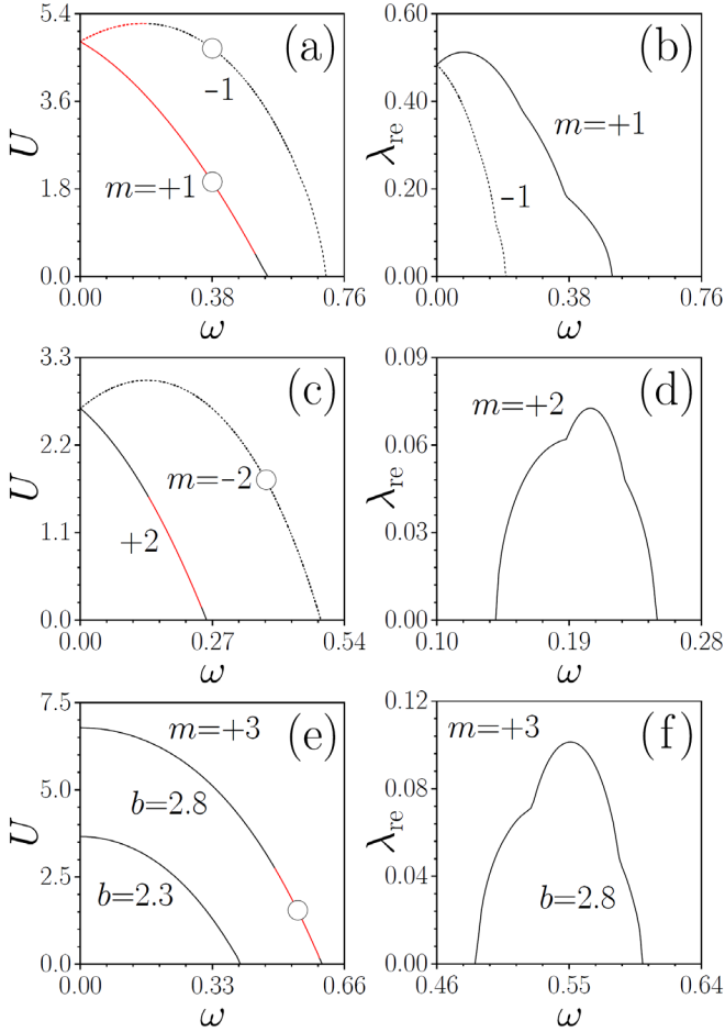
Fig. 3. Power (left) and maximal perturbation growth rate (right) versus rotation frequency \omega for m = \pm 1 solitons at b = 2.8 (a),(b), m = \pm 2 solitons at b = 2.3 (c),(d), and m = 3 solitons at b = 2.3 and b = 2.8 (e),(f). Stable branches are shown black, unstable ones are shown red. Dots correspond to solitons, whose propagation dynamics is depicted in Fig. 5.
