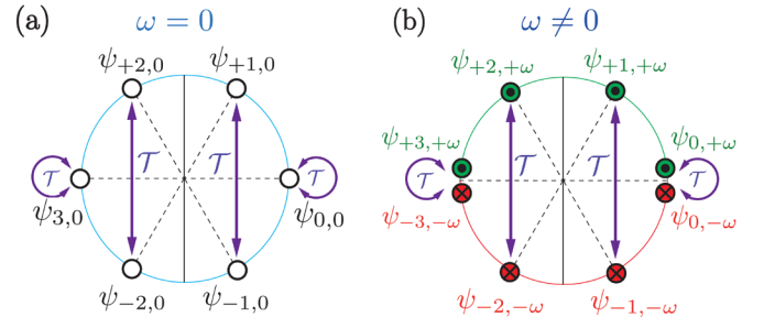
Fig. 1. Angular Bloch modes \psi_m as representations of the point group C_6 for exemplary array with N = 6 . They are described as the roots of unity e^{im\pi/3} in terms of their OAPM m . (a) For \omega = 0 (non-rotating case) the m = \pm 1, \pm 2 modes form degenerate doublets due to time reversal symmetry. (b) For \omega \neq 0 , time reversal is broken, which now connects an m mode with its partner -m with opposite value of \omega . A frequency value -\omega is represented by a red cross whereas a frequency value \omega is indicated by a green dot.
