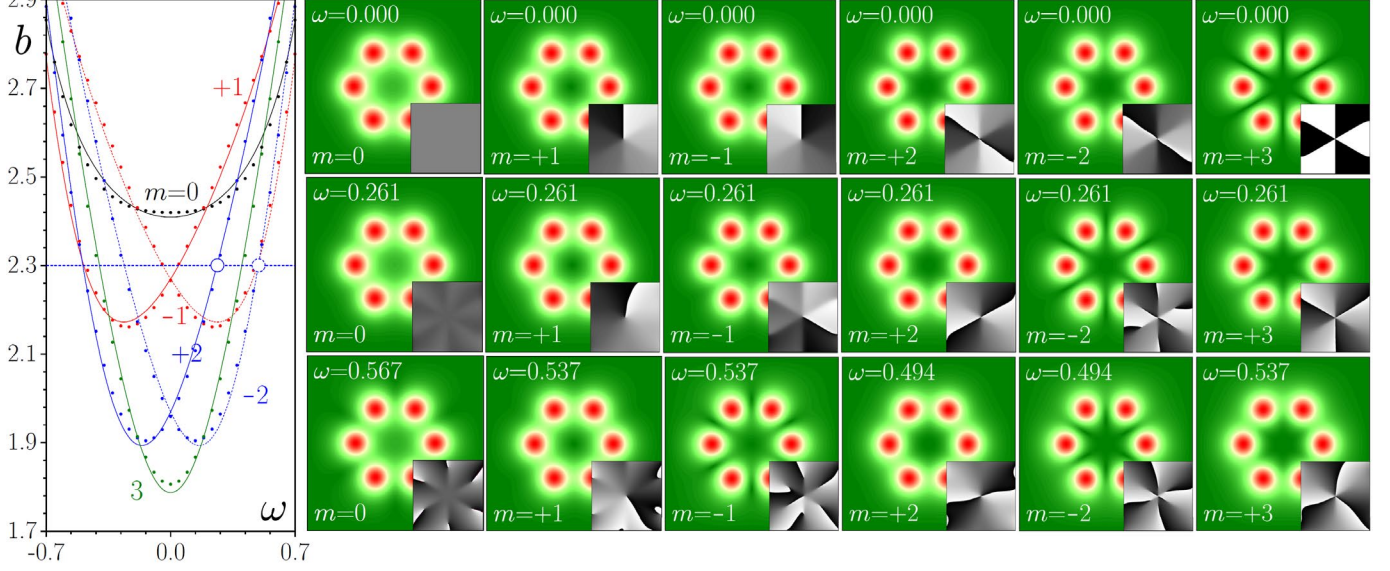
Fig. 2. Exact numerically calculated eigenvalues (lines) and their analytical approximation (dots) for linear modes of the rotating structure with N = 6 waveguides vs \omega and examples of modes ( |\psi| distributions and \arg(\psi) distributions in the insets) with different m, \omega values. Open blue circles indicate crossings of the horizontal dashed line b = 2.3 with m = \pm 2 mode families that occur at different frequencies.
