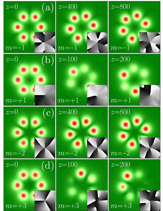
Fig. 5. Propagation of stable vortex solitons with m = -1 , b = 2.8 , \omega = 0.38 (a) and m = -2 , b = 2.3 , \omega = 0.38 (c), and decay of the unstable states with m = +1 , b = 2.8 , \omega = 0.38 (b), and m = +3 , b = 2.8 , \omega = 0.54 (d).
