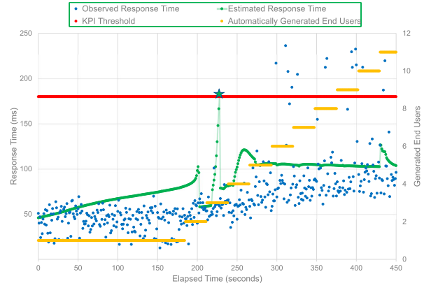
Fig. 3. Estimated Response Time versus Observed Response Time as a function of the number of Cassandra users.
