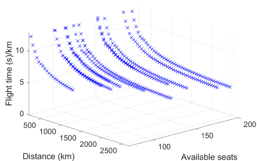
Figure 9. Flight gate-to-gate time (s) per kilometre vs. flight distance (km) and available seats.
