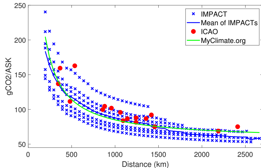
Figure 6. gCO 2 emissions per ASK vs. distance for different models of Category D.
