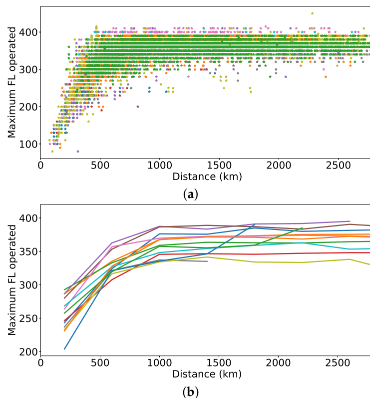
Figure 4. Flight levels operated for different aircraft types in Categories D and E. (a) Flight levels used per individual flight, as in the historical data (one day of operations). (b) Mean flight level grouped every 400 km.
