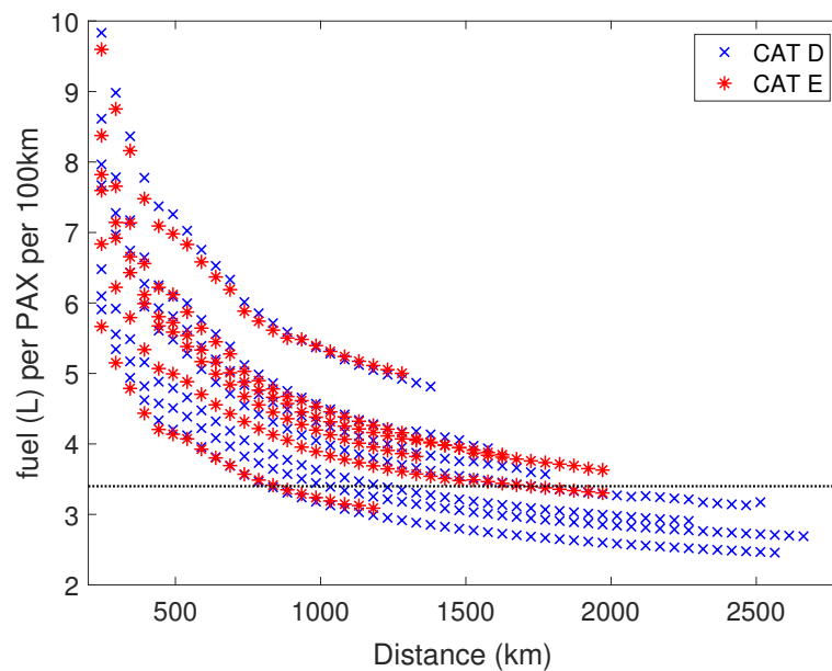
Figure 7. Fuel consumption (L) per passenger (assuming an 82.3% load factor and a PAX to freight factor of 96.1%) and per 100 km vs. flight distance.
