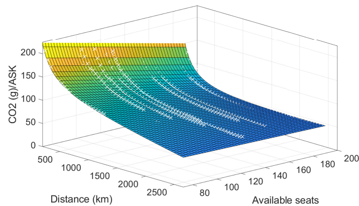
Figure 10. CO 2 emissions (g) per ASK vs. flight distance (km) and available seats and fitting surface.
