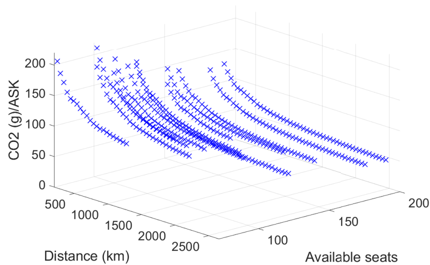
Figure 8. CO 2 emissions (g) per ASK vs. flight distance (km) and available seats.
