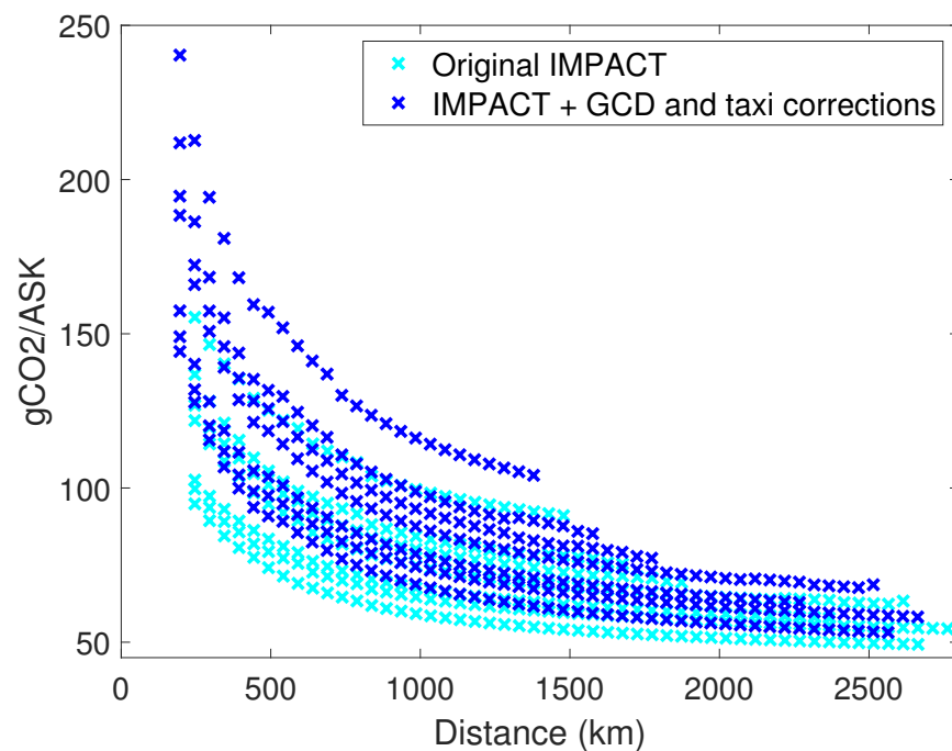
Figure 5. Effect of applying correction factors on the IMPACT results for Category D aircraft.
