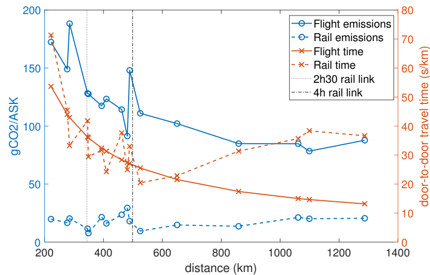
Figure 13. Comparison of total travel time and CO 2 emissions between train and flight for 16 European routes.
