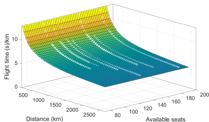
Figure 11. Flight gate-to-gate time (s) per kilometre vs. distance (km) and available seats and fitting surface.
