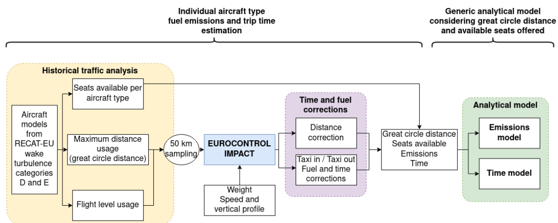
Figure 2. Methodology for developing emissions and time models.
