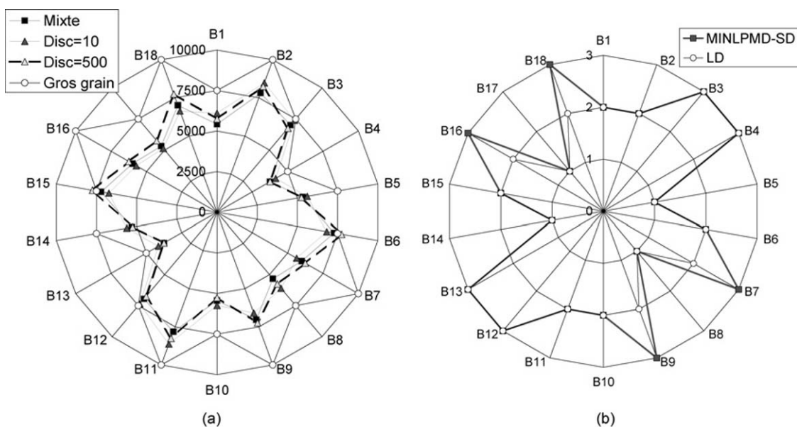
Figure 8. Batch stages volumes (a) and item number per stage (b) of example 5 solution, according to the discretization mode.
