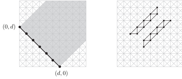
Fig. 3 Left: Illustrating Proposition 1. The shortest path from (0, d) to (d, 0) and the set A_d , which is in the shaded region. Right: Examples of horizontal and vertical MOP zigzags
