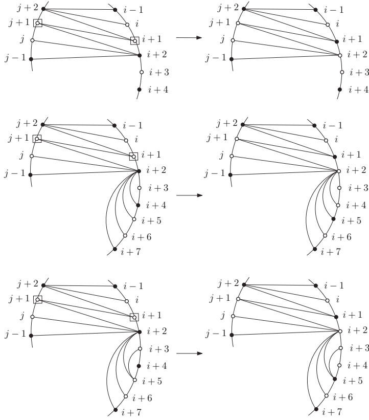
Fig. 15 Case (g). Squared vertices have the same coordinates. Top: Interchanging the colors of i + 1 and i + 2 . Middle and bottom: Interchanging the colors of i + 1 and i + 2 and the colors of i + 4 and i + 5
