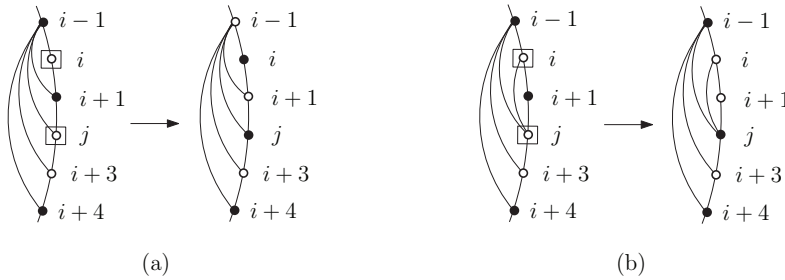
Fig. 11 Squared vertices have the same coordinates. Case (a): interchanging the colors of i and i - 1 , and j = i + 2 and i + 1 . Case (b): interchanging the colors of i + 1 and j = i + 2
