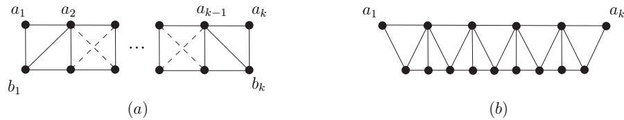
Fig. 1 (a) Given a 2-tree G with metric dimension 2, a minimal induced 2-connected subgraph containing the basis \{a_1, a_k\} , as claimed in [2]. (b) A 2-tree with metric basis \{a_1, a_k\} whose minimal induced 2-connected subgraph containing a_1 and a_k is different from the claimed subgraph in [2]
