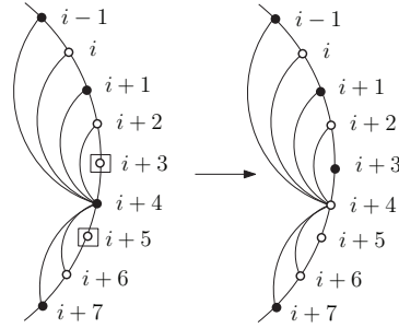
Fig. 13 Case (c). Squared vertices have the same coordinates. When i + 3 is not arranged by (S \setminus \{i + 2\}) \cup \{i + 1\} , the colors of i + 3 and i + 4 are interchanged
