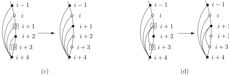
Fig. 12 Squared vertices have the same coordinates. Case (c): Interchanging the colors of i+1 and i+2 , when i+3 is arranged by (S \setminus \{i+2\}) \cup \{i+1\} . Case (d): Interchanging the colors of i+1 and i+2
