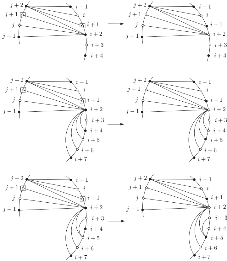
Fig. 16 Case (h). Squared vertices have the same coordinates. Top: Interchanging the colors of i+1 and i+2 . Middle and bottom: Interchanging the colors of i+1 and i+2 and the colors of i+4 and i+5
