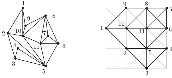
Fig. 2 Left: A graph G with metric basis S = \{1, 3\} . The metric coordinates of the vertices are: r(1|S) = (0, 2) , r(2|S) = (1, 1) , r(3|S) = (2, 0) , r(4|S) = (3, 1) , r(5|S) = (2, 1) , r(6|S) = (3, 2) , r(7|S) = (3, 3) , r(8|S) = (2, 3) , r(9|S) = (1, 3) , r(10|S) = (1, 2) and r(11|S) = (2, 2) . Right: The representation G^* of G as a subgraph of P_n \boxtimes P_n with respect to S . Vertex v in G is mapped to vertex v^* in G^* such that the cartesian coordinates of v^* are the metric coordinates of v
