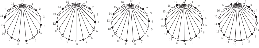
Fig. 8 The set of black vertices is a metric basis of the fans of order 15, 16, 17, 18 and 19
