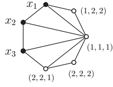
Fig. 7 The fan F_{1,6} . Black vertices form a metric basis S . For a vertex not in S , its metric coordinates are given
