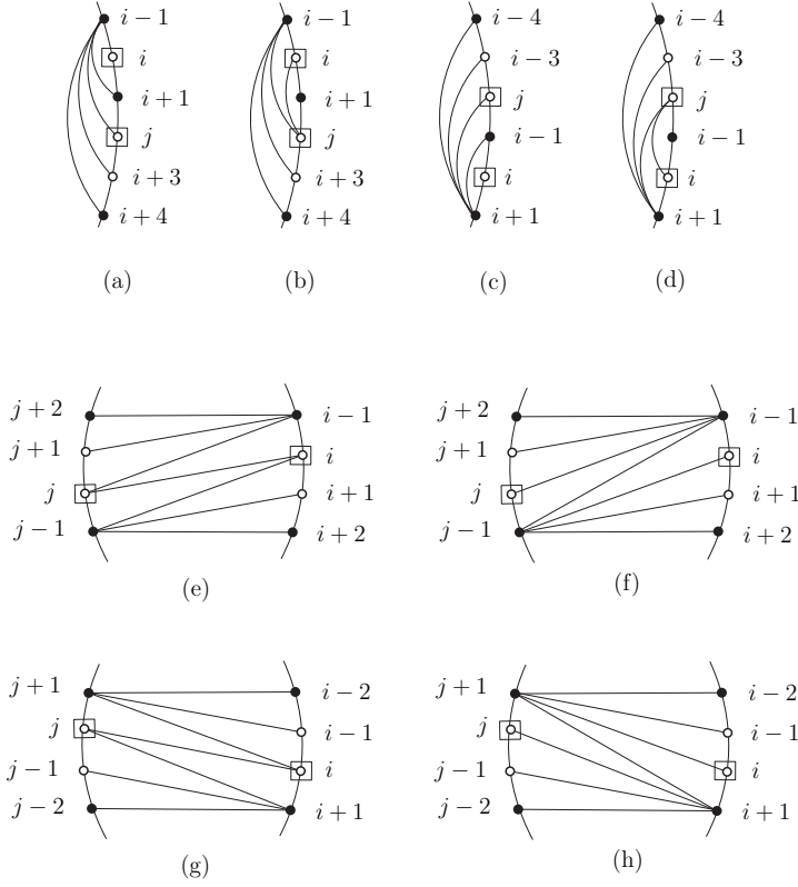
Fig. 10 The eight cases in which two white vertices i and j , squared in the figure, are not resolved by black vertices
