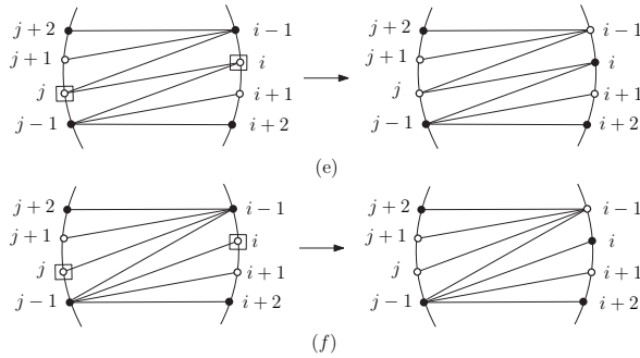
Fig. 14 Cases (e) and (f): squared vertices have the same coordinates. Interchanging the colors of i-1 and i
