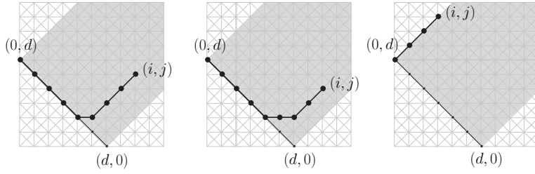
Fig. 5 A (0, d) - (i, j) path of length i when i - j and d have distinct parity (left); when i - j and d have the same parity and i - j \neq -d (center) and when i - j = -d (right)
