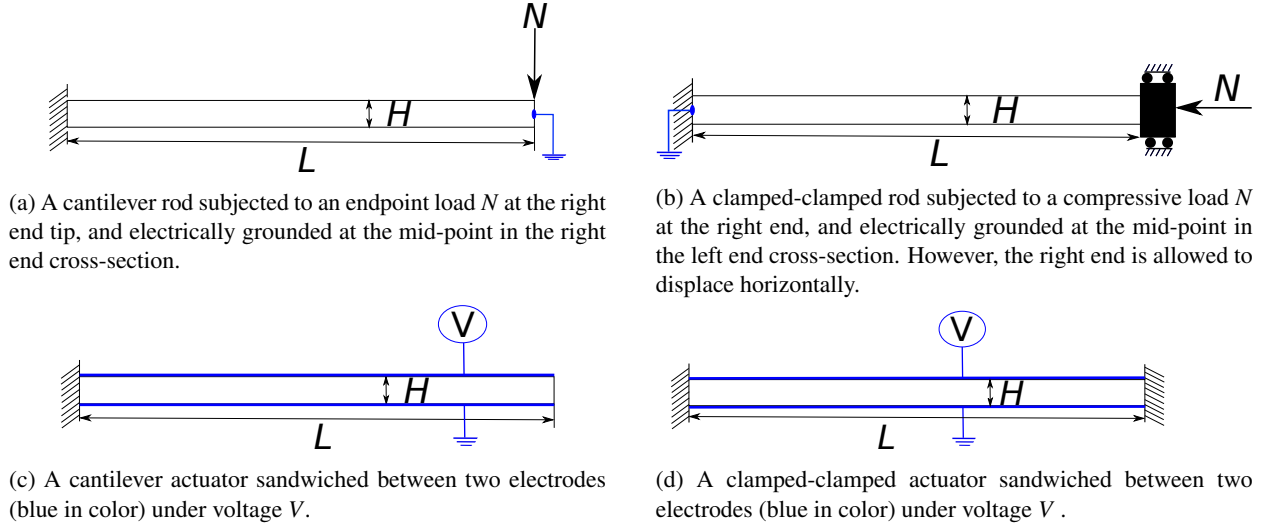
Figure 3: A schematic of flexoelectric rod under external mechanical load or external voltage.
