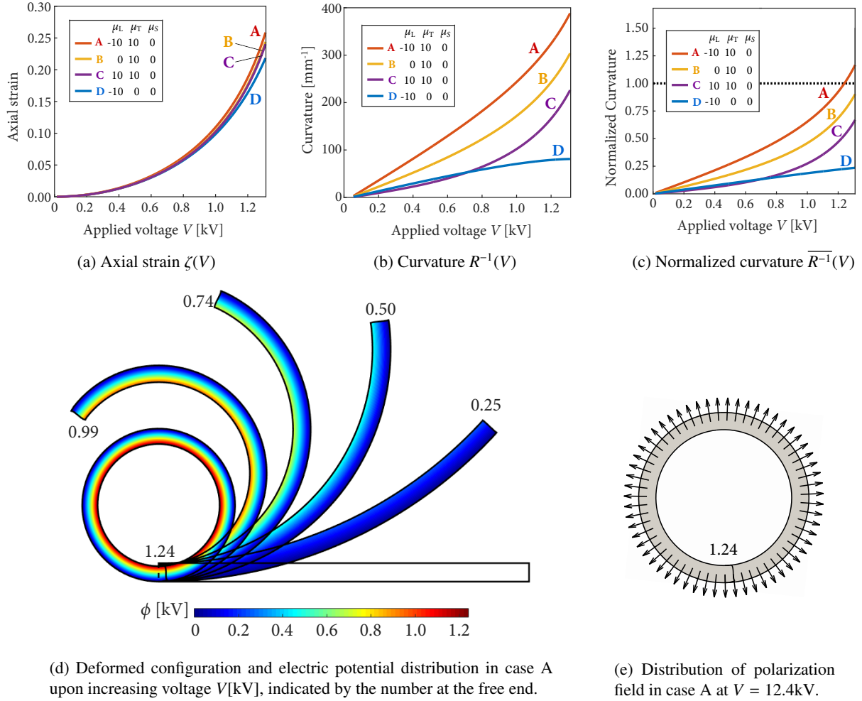
Figure 8: Actuation of Neo-Hookean cantilever rod with different flexoelectric tensors (expressed in nJ/Vm)
