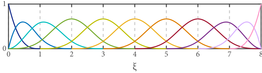
Figure 1: Univariate open uniform B-spline basis of degree p = 3 . Each basis function is a smooth ( C^{p-1} ) piece-wise polynomial on a compact ( \leq p + 1 ) support. Multivariate B-spline bases are constructed by means of the tensor product of multiple univariate bases.
