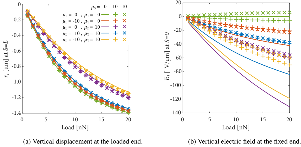
Figure 5: Electromechanical response of Neo-Hookean cantilever flexoelectric sensor under bending, with different flexoelectric tensors (expressed in \text{nJ}/\text{Vm} ).
