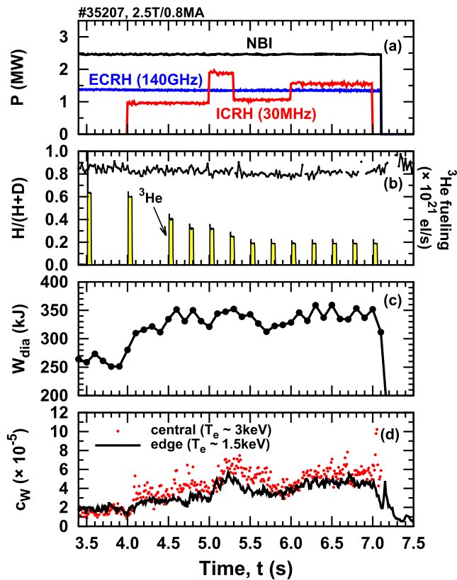
Figure 12. Overview of AUG pulse #35207 with far off-axis ICRH heating of ^3\text{He} ions in H-D plasmas (2.5 T/0.8 MA): (a) NBI, ECRH and ICRH heating power; (b) H/(H + D) ratio measured by NPA and ^3\text{He} fuelling blips; (c) plasma stored energy; (d) tungsten concentration (core and edge).
