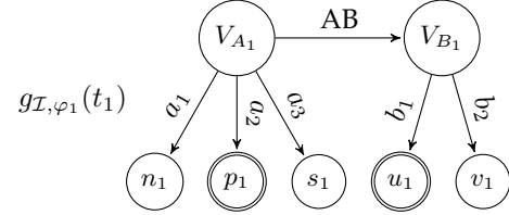
Fig. 4: Contained source query, execution and global instance of the global query from Figure 2
