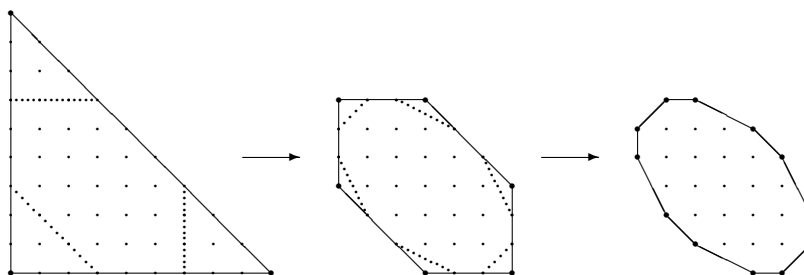
FIGURE 1. \mathbb{C}P^2 , \mathbb{C}P^2\#3\overline{\mathbb{C}P}^2 , and \mathbb{C}P^2\#9\overline{\mathbb{C}P}^2 .
