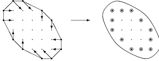
FIGURE 2. Nodal trades on \mathbb{C}P^2 \# 9\overline{\mathbb{C}P^2} .
