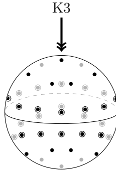
FIGURE 3. K3 surface as a singular fiber bundle over the sphere.
