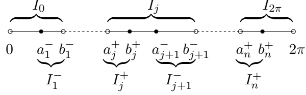
FIGURE 4. Intervals along a focus-focus fiber.
