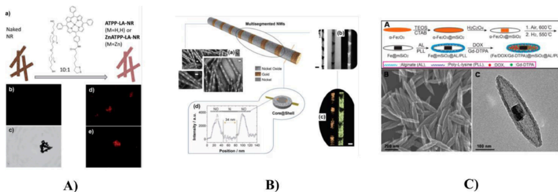
Fig. 6. Functionalization strategies employed to modify the surface of micro/nanomotors. (A) Scheme showing the functionalization of nanorods with porphyrins for photodynamic therapy. And fluorescence microscope images showing functionalized and non-functionalized nanomotors. Reproduced with permission from reference [92]. Copyright 2017, Royal Society of Chemistry. (B) Oxidation treatment of Ni segments in multisegmented Ni-Au nanorods to confer biocompatibility through the formation of nickel oxide surface layers. Reproduced with permission from reference [97]. Copyright 2018, Wiley. (C) Magnetic nanocapsules consisting of an hematite core and a mesoporous silica shell containing doxorubicin as a model drug. The capsules were functionalized with multiple polyelectrolyte layers of poly-L-lysine and sodium alginate to thigh drug delivery control. Reproduced with permission from reference [98]. Copyright 2014, American Chemical Society.
