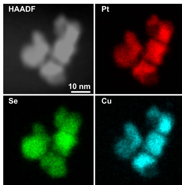
Figure 5. HAADF-STEM image and corresponding elemental maps by STEM EDS of Pt-Cu-Se_C.
