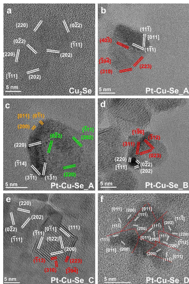
Figure 7. HRTEM images of representative NPs of \text{Cu}_2\text{Se} (panel a), Pt-Cu-Se_A (panels b, c), Pt-Cu-Se_B (panel d), Pt-Cu-Se_C (panel e), Pt-Cu-Se_D (panel f). Different phases in panels B-E are depicted in false colors as indicated: Phase A (main) \rightarrow white; Phase B (main) \rightarrow red, Phase A (minor) \rightarrow green; Phase B (minor) \rightarrow orange.
