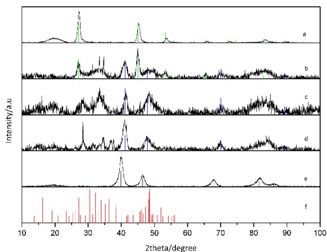
Figure 2. XRD patterns of a) \text{Cu}_{2-x}\text{Se} NPs, b) sample A (ratio Pt:Cu 0.1), c) sample B (ratio Pt:Cu 0.2), d) sample C (ratio Pt:Cu 0.65) and, e) sample D (ratio Pt:Cu 1.6). Reference patterns of cubic \text{Cu}_2\text{Se} (JCPDS 088-2043) in green; cubic CuPt (JCPDS 048-1549) in blue; cubic Pt (JCPDS 087-0640) in black, and monoclinic \text{Pt}_5\text{Se}_4 (JCPDS 00-031-0950) in red.
