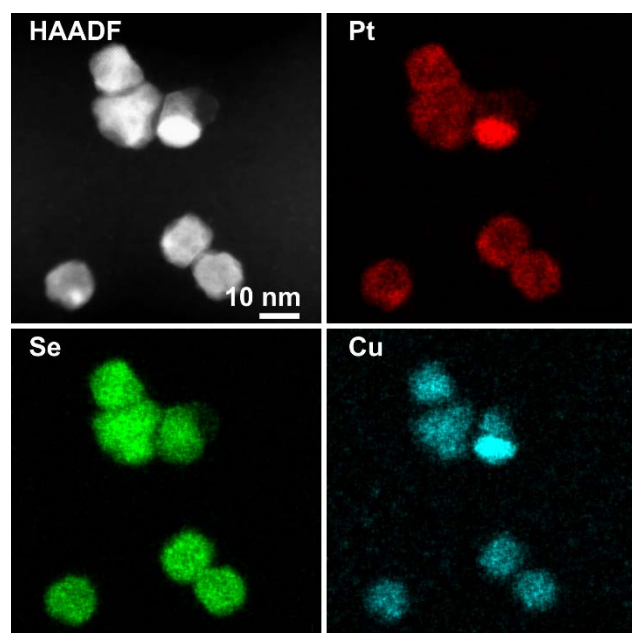
Figure 4. HAADF-STEM image and corresponding elemental maps by STEM EDS of Pt-Cu-Se_B.
