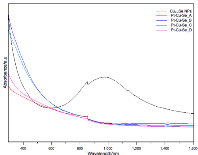
Figure 8. UV-Vis-NIR absorption spectra of \text{Cu}_{2-x}\text{Se} and Pt-Cu-Se_A-D samples.
