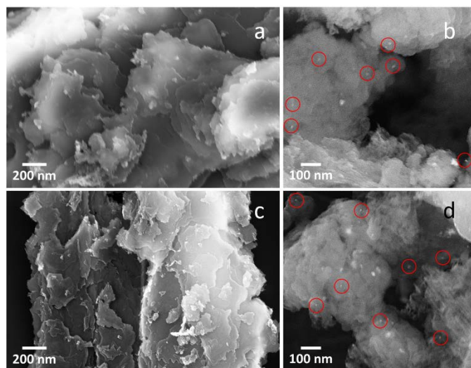
Figure 9. SEM micrographs of a,b) Pt-Cu-Se_B/ g\text{-C}_3\text{N}_4 and, c,d) Pt-Cu-Se_C/ g\text{-C}_3\text{N}_4 nanocomposites. Red circles indicate the position of Pt-Cu-Se_X NPs.
