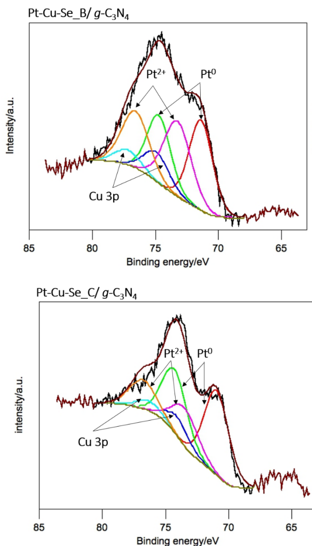
Figure 10. X-ray photoelectron spectra of the Pt 4f core level for Pt-Cu-Se_B/ g\text{-C}_3\text{N}_4 and Pt-Cu-Se_C/ g\text{-C}_3\text{N}_4 nanocomposites, and corresponding deconvolutions.
