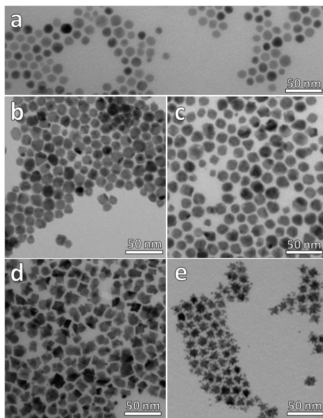
Figure 1. TEM micrographs of a) \text{Cu}_{2-x}\text{Se} NPs, b) sample A (ratio Pt:Cu 0.1), c) sample B (ratio Pt:Cu 0.2), d) sample C (ratio Pt:Cu 0.65) and, e) sample D (ratio Pt:Cu 1.6).
