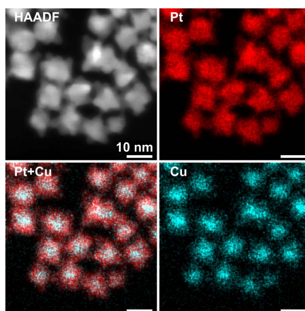
Figure 6. HAADF-STEM image and corresponding elemental maps by STEM EDS of Pt-Cu-Se_D.
