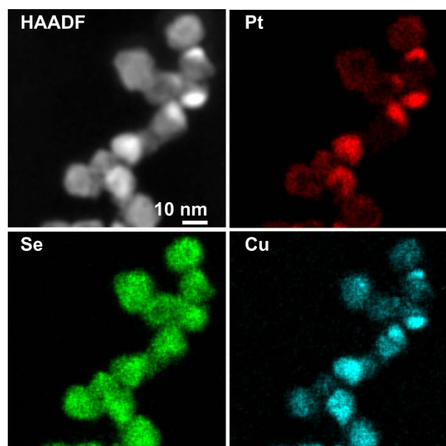
Figure 3. HAADF-STEM image and corresponding elemental maps by STEM EDS of Pt-Cu-Se_A.
