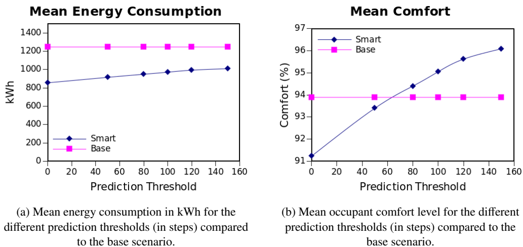
Figure 9: Energy and comfort comparison results between the smart and base scenario.
