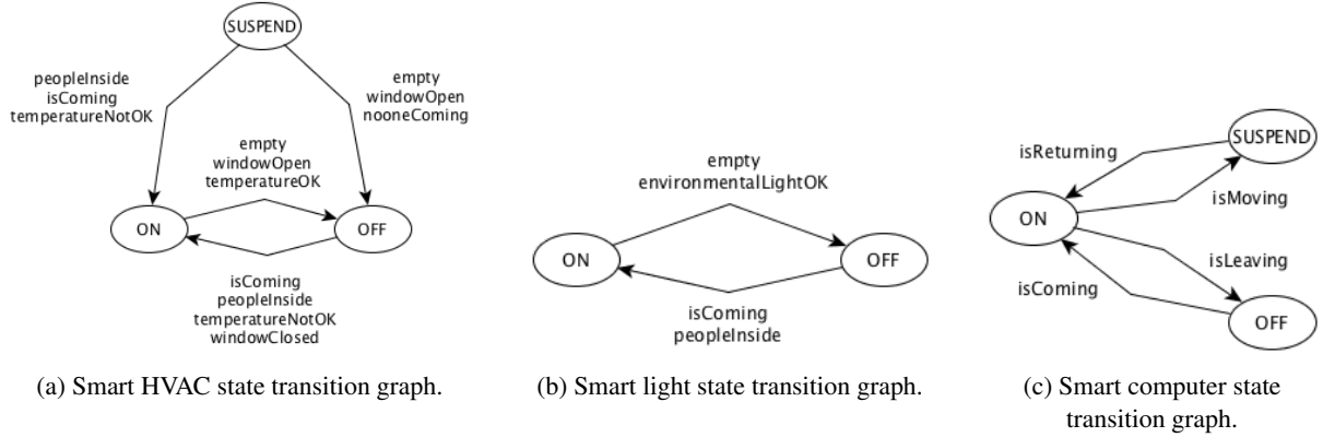
Figure 5: State transition graphs for the monitored elements.
