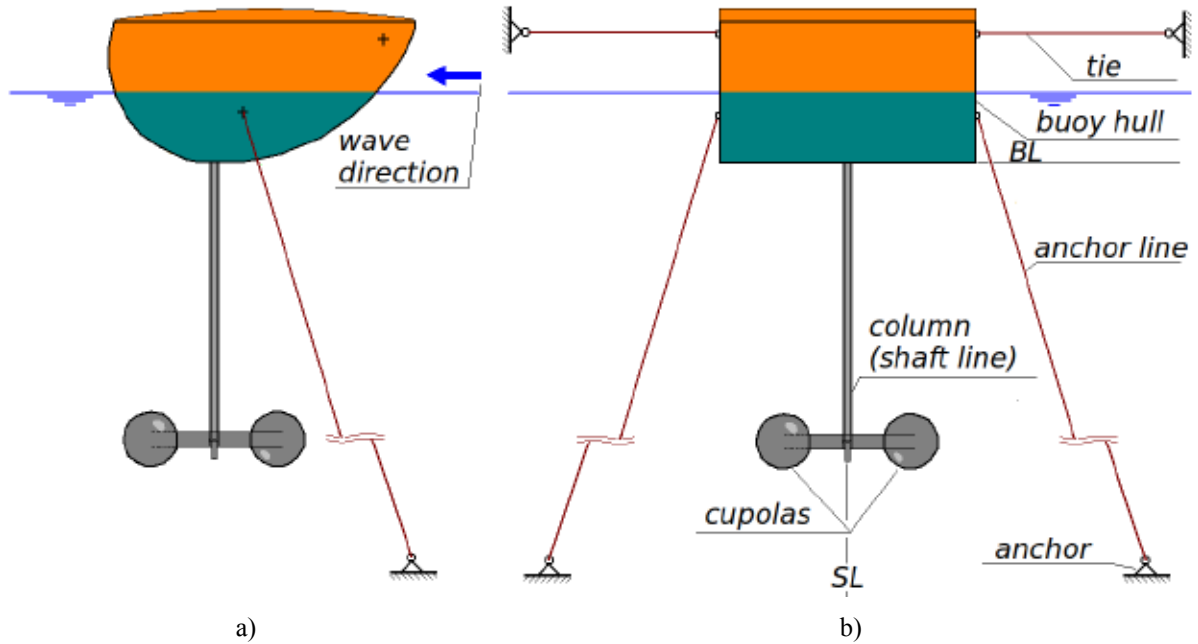
Figure 2: a) Sketch of anchoring system
