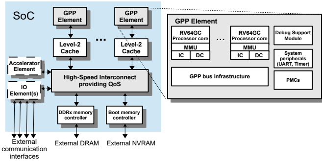
Fig. 1. Baseline SELENE SoC architecture.
