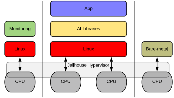
Fig. 2. SELENE SW Architecture.
