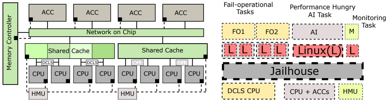
Fig. 3. Particular instance of SELENE platform. Hardware view (left) and logical view (right).
