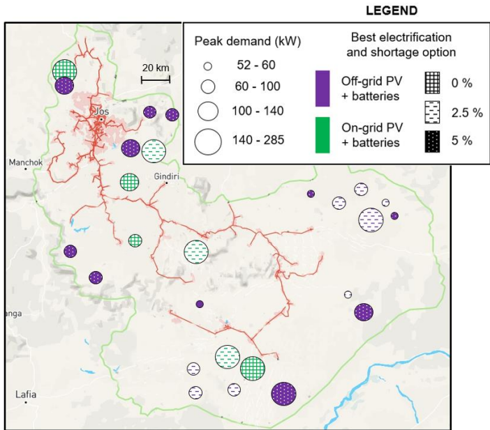
Figure 4. Final electrification alternative selected for each settlement (background image from http://rep-nigeria.integration.org/# )
