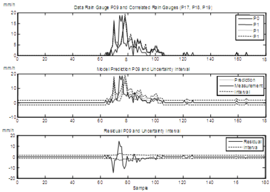
Fig. 18 Fault in rain-gauge P_{09} in the 15/11/2001 rain-scenario
