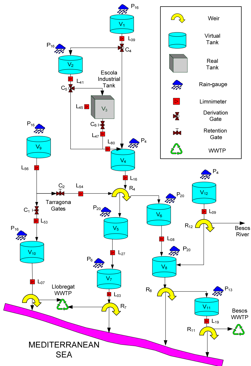
Fig. 7. Virtual reservoir model of the portion of Barcelona network considered
