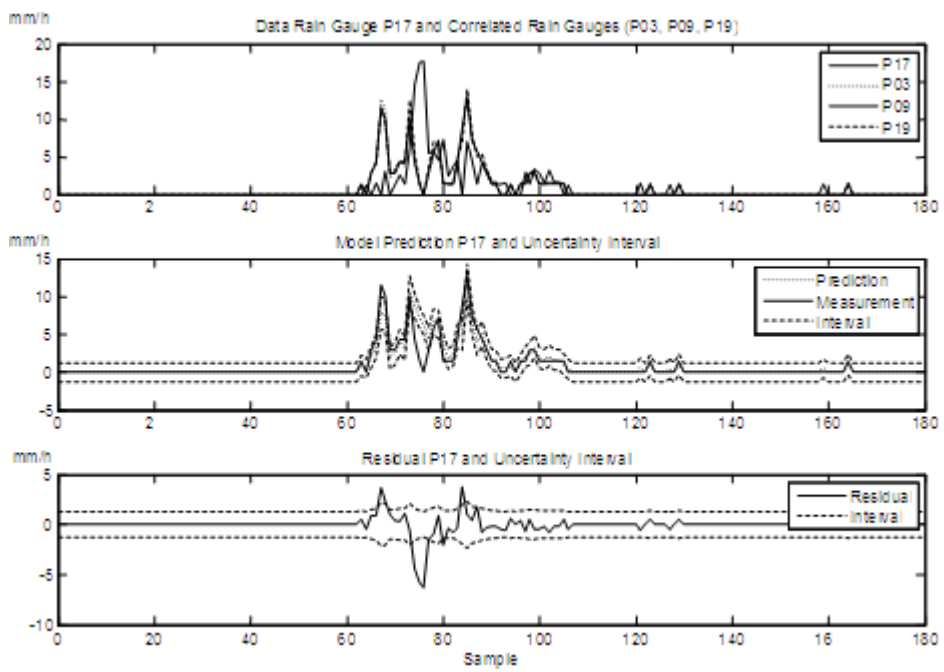
Fig. 19. Fault in rain-gauge P_{09} in the 15/11/2001 rain-scenario
