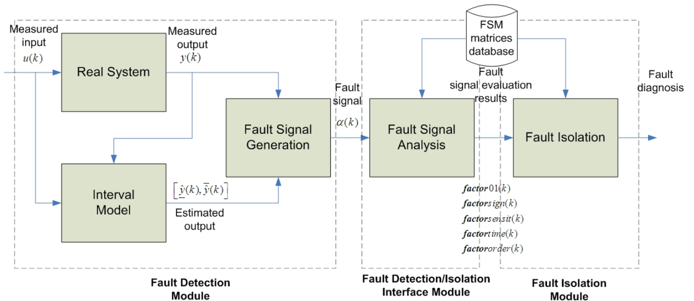
Fig. 4. FDI proposed scheme
